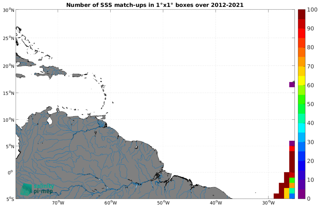
Figure 5: Number of SSS match-ups between TSG (Polarstern) SSS and the SMOS SSS L4 v2 - Daily (BEC) SSS product for the Amazon and Orinoco river plumes Pi-MEP region over 1^{\circ} \times 1^{\circ} boxes and for the full satellite product period.
