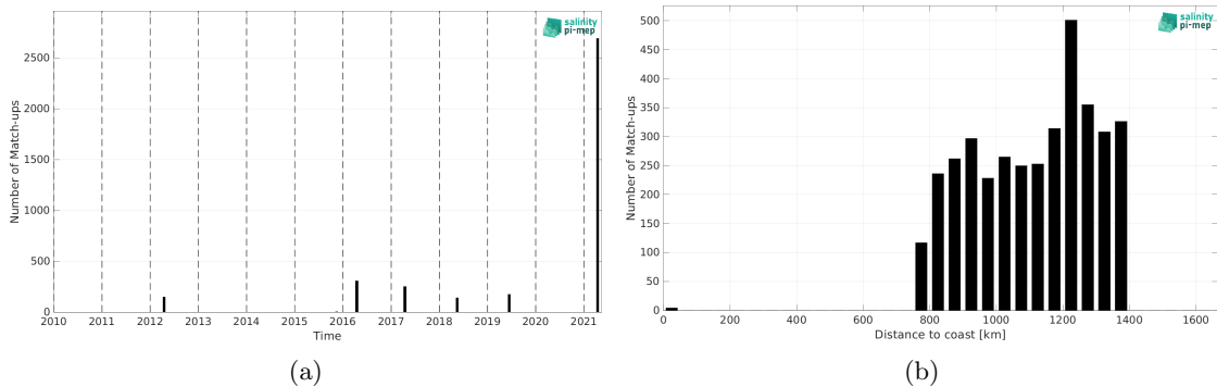
Figure 2: Number of match-ups between TSG (Polarstern) and SMOS SSS L4 v2 - Daily (BEC) SSS as a function of time (a) and as function of the distance to coast (b) over the Amazon and Orinoco river plumes Pi-MEP region and for the full satellite product period.
