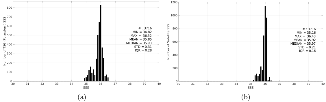
Figure 3: Histograms of SSS from TSG (Polarstern) (a) and SMOS SSS L4 v2 - Daily (BEC) (b) considering all match-up pairs per bins of 0.1 over the Amazon and Orinoco river plumes Pi-MEP region and for the full satellite product period.
