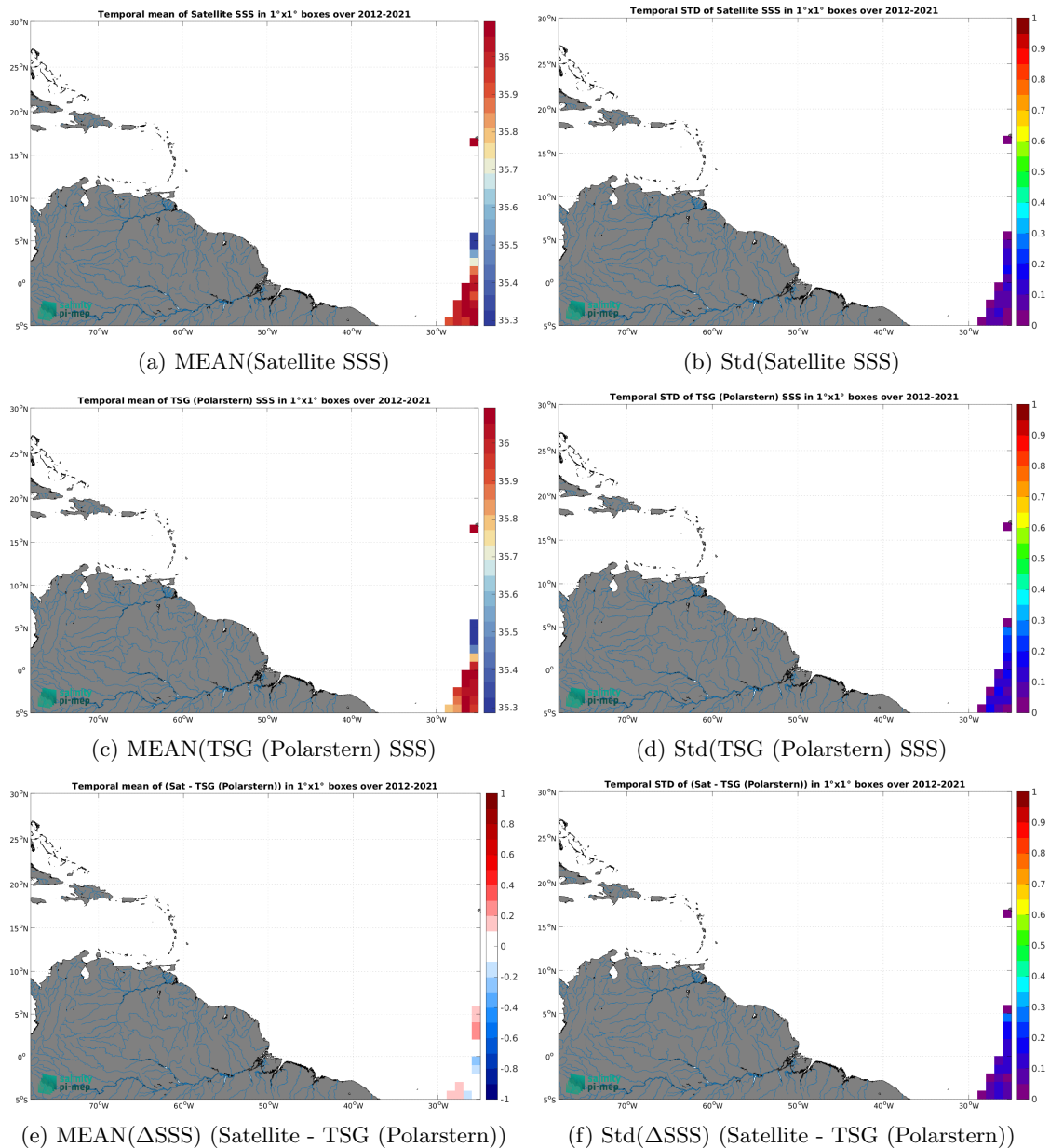
Figure 7: Temporal mean (left) and Std (right) of SSS from SMOS SSS L4 v2 - Daily (BEC) (top), TSG (Polarstern) (middle), and of \Delta SSS (Satellite - TSG (Polarstern)). Only match-up pairs are used to generate these maps.
