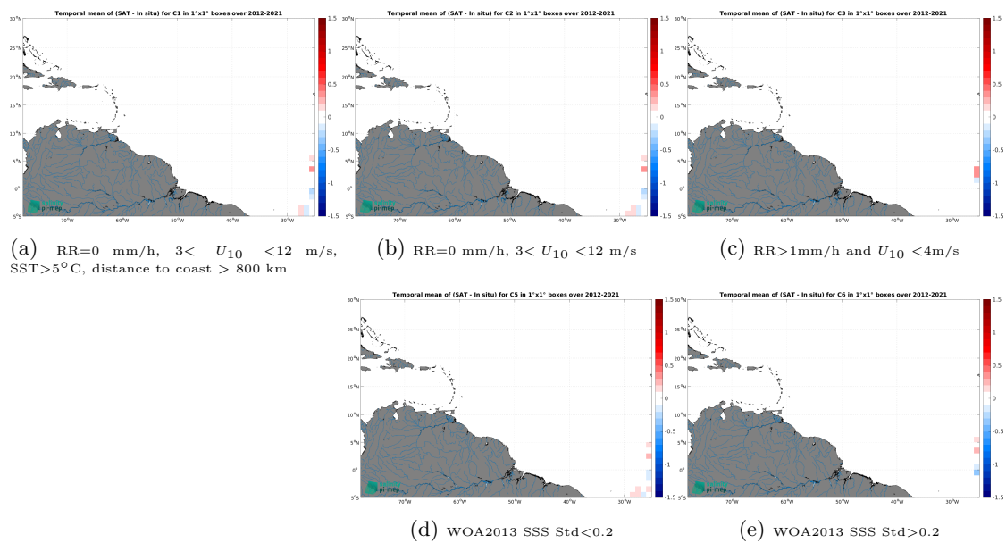
Figure 14: Temporal mean gridded over spatial boxes of size 1^\circ \times 1^\circ of \Delta SSS (SMOS SSS L4 v2 - Daily (BEC) - TSG (Polarstern)) for 5 different subdatasets corresponding to:RR=0 mm/h, 3 < U_{10} < 12 m/s, SST >5^\circ\text{C} , distance to coast > 800 km (a), RR=0 mm/h, 3 < U_{10} < 12 m/s (b), RR >1 mm/h and U_{10} < 4 m/s (c), WOA2013 SSS Std <0.2 (d), WOA2013 SSS Std >0.2 (e).
