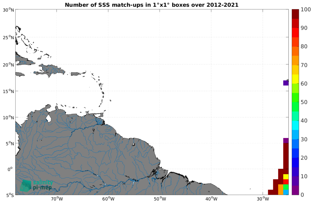
Figure 4: Number of SSS match-ups between TSG (Polarstern) SSS and the SMOS SSS L4 v2 - Daily (BEC) SSS product for the Amazon and Orinoco river plumes Pi-MEP region over 1^{\circ} \times 1^{\circ} boxes and for the full satellite product period.
