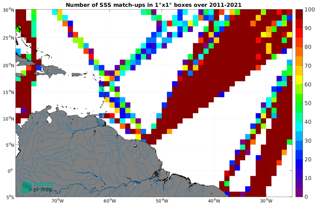
Figure 4: Number of SSS match-ups between TSG (LEGOS-DM) SSS and the SMOS SSS L4 v2 - Daily (BEC) SSS product for the Amazon and Orinoco river plumes Pi-MEP region over 1^{\circ} \times 1^{\circ} boxes and for the full satellite product period.
