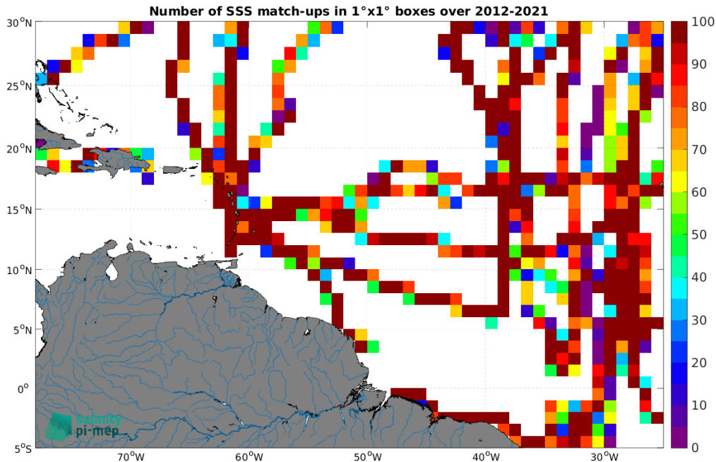
Figure 5: Number of SSS match-ups between TSG (GOSUD-Sailing-ship) SSS and the SMOS SSS L4 v2 - Daily (BEC) SSS product for the Amazon and Orinoco river plumes Pi-MEP region over 1^\circ \times 1^\circ boxes and for the full satellite product period.
