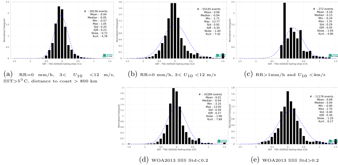
Figure 15: Normalized histogram of \Delta SSS (SMOS SSS L4 v2 - Daily (BEC) - TSG (GOSUD-Sailing-ship)) for 5 different subdatasets corresponding to: RR=0 mm/h, 3 < U_{10} < 12 m/s, SST>5°C, distance to coast > 800 km (a), RR=0 mm/h, 3 < U_{10} < 12 m/s (b), RR>1mm/h and U_{10} < 4 m/s (c), WOA2013 SSS Std<0.2 (d), WOA2013 SSS Std>0.2 (e).
