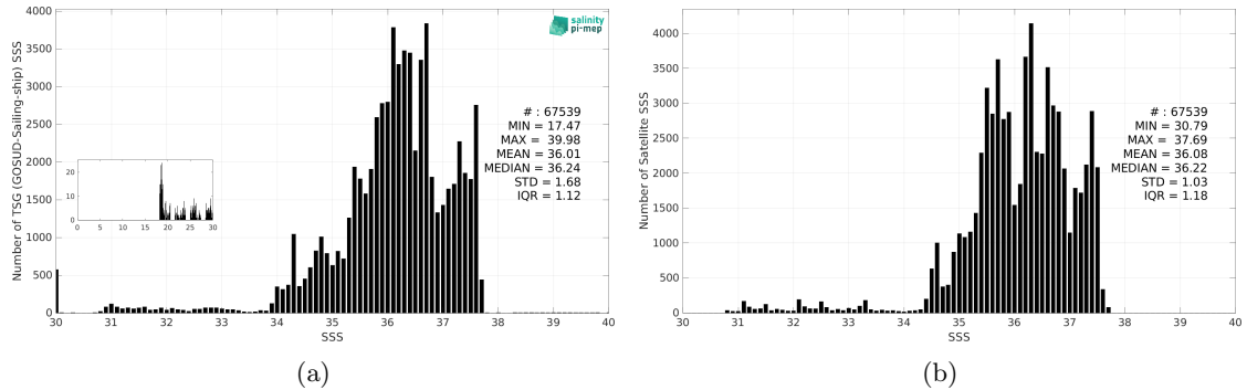
Figure 3: Histograms of SSS from TSG (GOSUD-Sailing-ship) (a) and SMOS SSS L4 v2 - Daily (BEC) (b) considering all match-up pairs per bins of 0.1 over the Amazon and Orinoco river plumes Pi-MEP region and for the full satellite product period.
