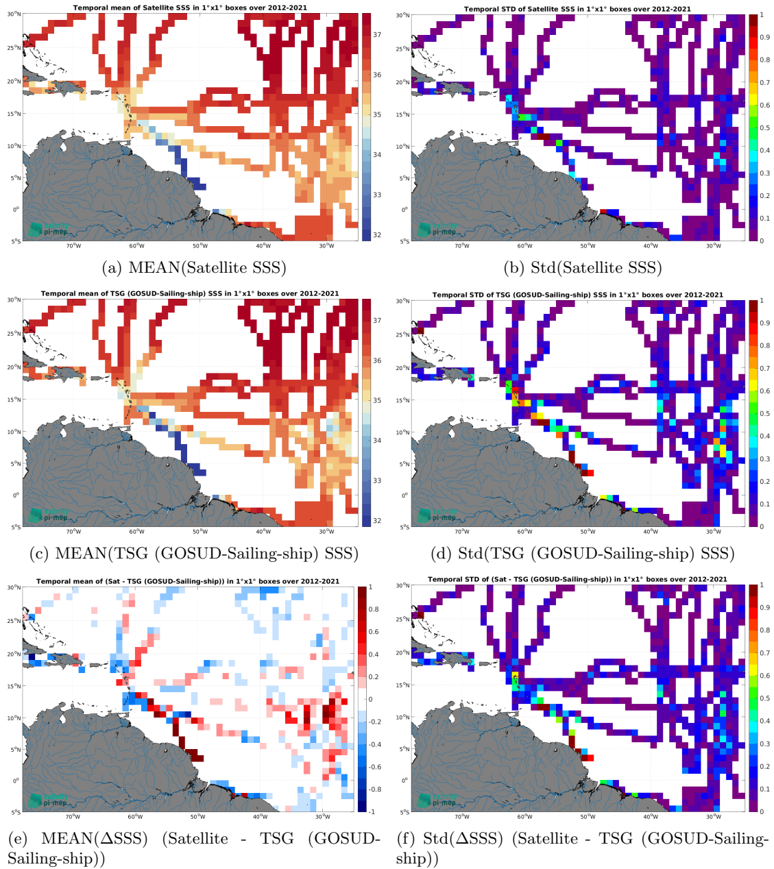
Figure 7: Temporal mean (left) and Std (right) of SSS from SMOS SSS L4 v2 - Daily (BEC) (top), TSG (GOSUD-Sailing-ship) (middle), and of \Delta SSS (Satellite - TSG (GOSUD-Sailing-ship)). Only match-up pairs are used to generate these maps.
