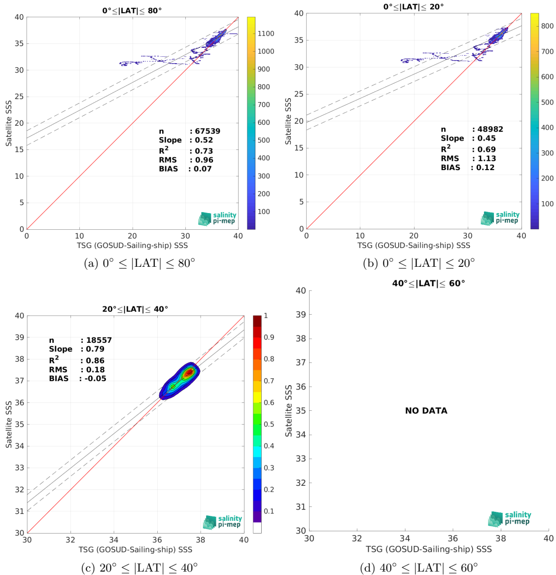
Figure 10: Contour maps of the concentration of SMOS SSS L4 v2 - Daily (BEC) SSS (y-axis) versus TSG (GOSUD-Sailing-ship) SSS (x-axis) at match-up pairs for different latitude bands. For each plot, the red line shows x=y . The black thin and dashed lines indicate a linear fit through the data cloud and the \pm 95\% confidence levels, respectively. The number match-up pairs n , the slope and R^2 coefficient of the linear fit, the root mean square (RMS) and the mean bias between satellite and in situ data are indicated for each latitude band in each plots.
