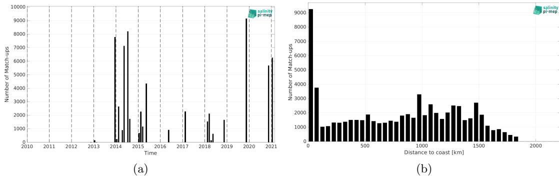
Figure 2: Number of match-ups between TSG (GOSUD-Sailing-ship) and SMOS SSS L4 v2 - Daily (BEC) SSS as a function of time (a) and as function of the distance to coast (b) over the Amazon and Orinoco river plumes Pi-MEP region and for the full satellite product period.
