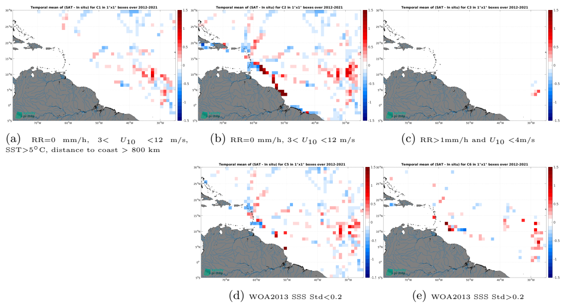
Figure 14: Temporal mean gridded over spatial boxes of size 1^\circ \times 1^\circ of \Delta SSS (SMOS SSS L4 v2 - Daily (BEC) - TSG (GOSUD-Sailing-ship)) for 5 different subdatasets corresponding to:RR=0 mm/h, 3 < U_{10} < 12 m/s, SST >5^\circ\text{C} , distance to coast > 800 km (a), RR=0 mm/h, 3 < U_{10} < 12 m/s (b), RR >1 mm/h and U_{10} < 4 m/s (c), WOA2013 SSS Std <0.2 (d), WOA2013 SSS Std >0.2 (e).
