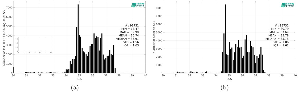
Figure 2: Histograms of SSS from TSG (GOSUD-Sailing-ship) (a) and SMOS SSS L4 v2 - Daily (BEC) (b) considering all match-up pairs per bins of 0.1 over the Amazon and Orinoco river plumes Pi-MEP region and for the full satellite product period.
