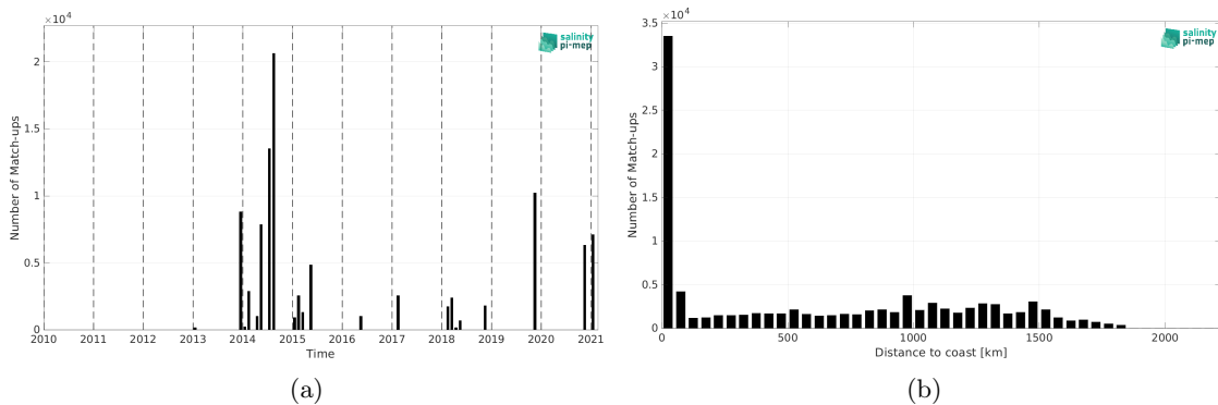
Figure 1: Number of match-ups between TSG (GOSUD-Sailing-ship) and SMOS SSS L4 v2 - Daily (BEC) SSS as a function of time (a) and as function of the distance to coast (b) over the Amazon and Orinoco river plumes Pi-MEP region and for the full satellite product period.
