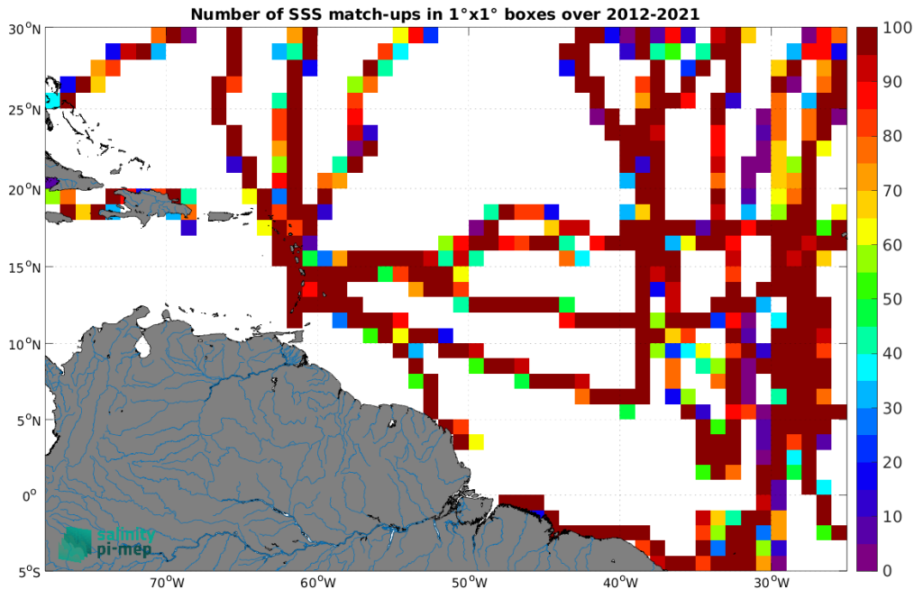
Figure 4: Number of SSS match-ups between TSG (GOSUD-Sailing-ship) SSS and the SMOS SSS L4 v2 - Daily (BEC) SSS product for the Amazon and Orinoco river plumes Pi-MEP region over 1°×1° boxes and for the full satellite product period.
