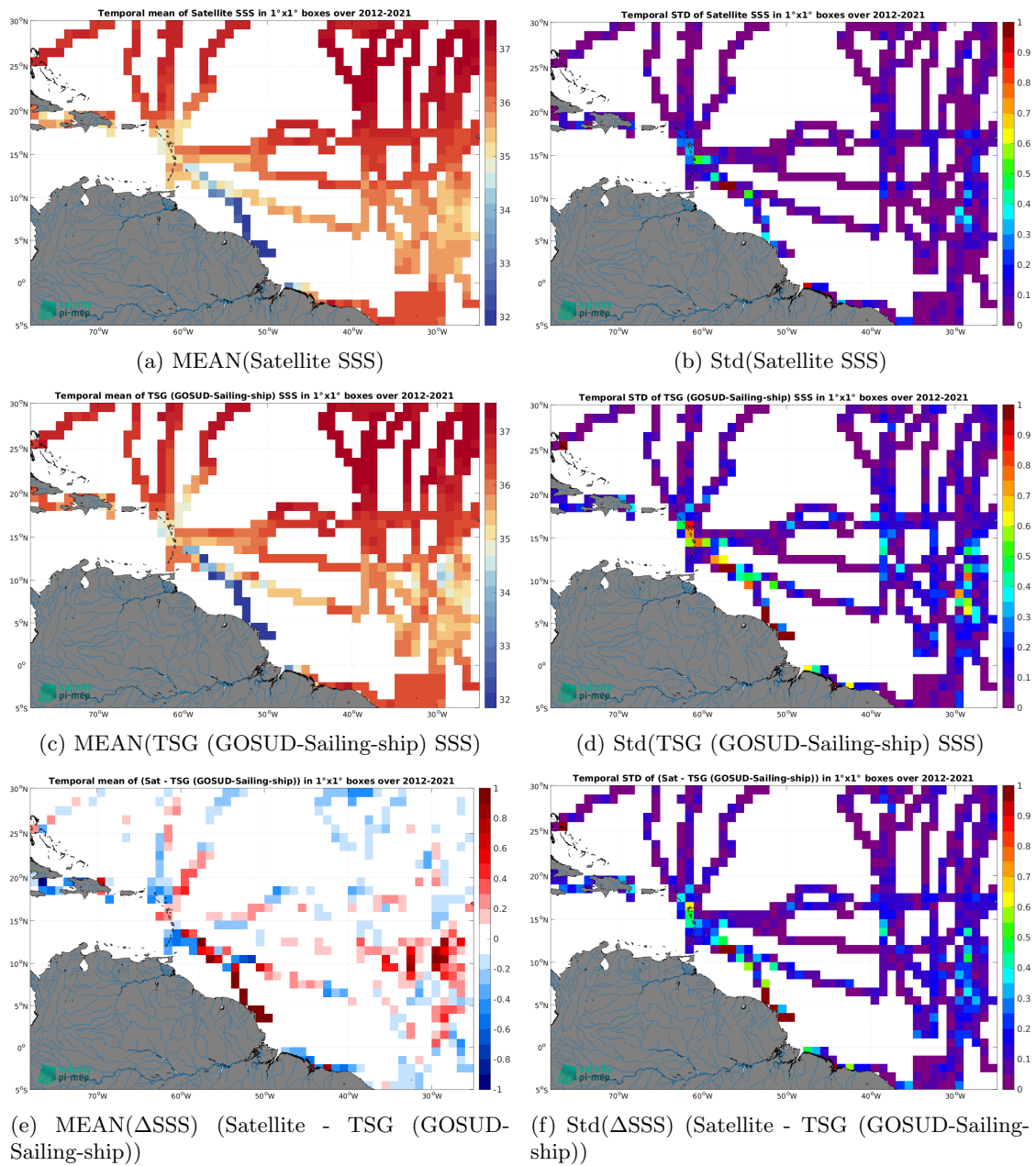
Figure 6: Temporal mean (left) and Std (right) of SSS from SMOS SSS L4 v2 - Daily (BEC) (top), TSG (GOSUD-Sailing-ship) (middle), and of \Delta SSS (Satellite - TSG (GOSUD-Sailing-ship)). Only match-up pairs are used to generate these maps.
