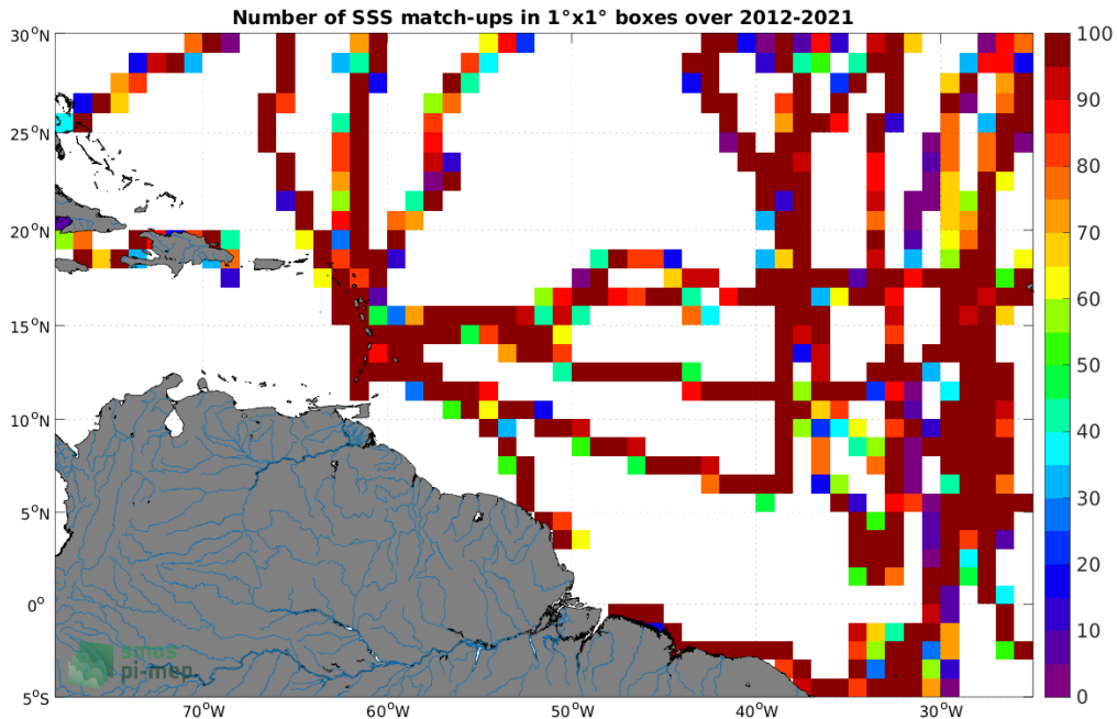
Figure 4: Number of SSS match-ups between TSG (GOSUD-Sailing-ship) SSS and the SMOS SSS L4 v2 - Daily (BEC) SSS product for the Amazon and Orinoco river plumes Pi-MEP region over 1^\circ \times 1^\circ boxes and for the full satellite product period.
