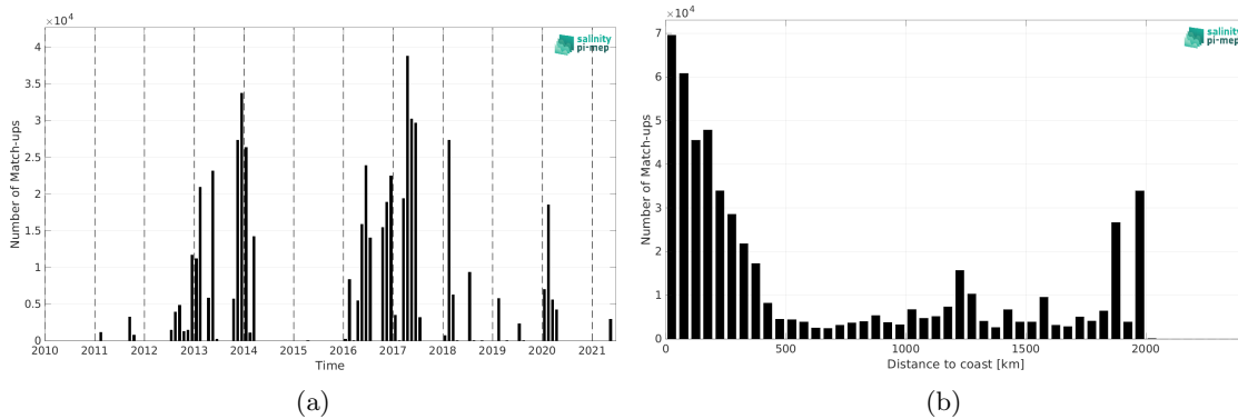
Figure 2: Number of match-ups between TSG (GOSUD-Research-vessel) and SMOS SSS L4 v2 - Daily (BEC) SSS as a function of time (a) and as function of the distance to coast (b) over the Amazon and Orinoco river plumes Pi-MEP region and for the full satellite product period.
