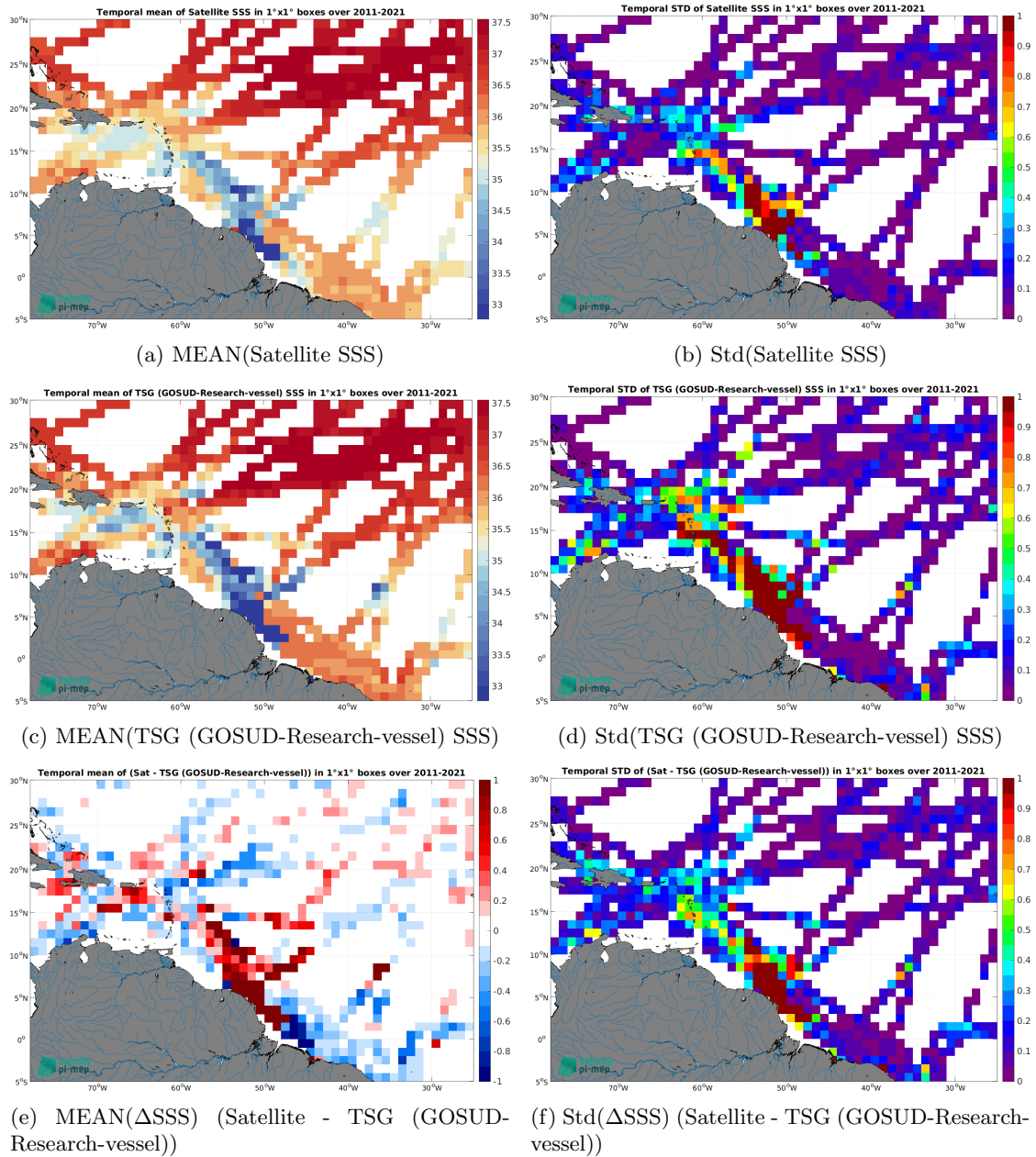
Figure 7: Temporal mean (left) and Std (right) of SSS from SMOS SSS L4 v2 - Daily (BEC) (top), TSG (GOSUD-Research-vessel) (middle), and of \Delta SSS (Satellite - TSG (GOSUD-Research-vessel)). Only match-up pairs are used to generate these maps.
