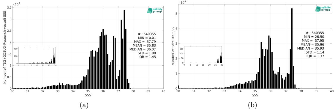
Figure 3: Histograms of SSS from TSG (GOSUD-Research-vessel) (a) and SMOS SSS L4 v2 - Daily (BEC) (b) considering all match-up pairs per bins of 0.1 over the Amazon and Orinoco river plumes Pi-MEP region and for the full satellite product period.
