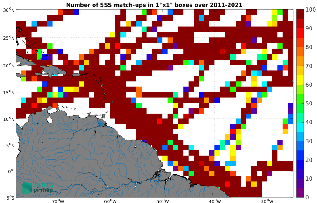
Figure 5: Number of SSS match-ups between TSG (GOSUD-Research-vessel) SSS and the SMOS SSS L4 v2 - Daily (BEC) SSS product for the Amazon and Orinoco river plumes Pi-MEP region over 1^\circ \times 1^\circ boxes and for the full satellite product period.
