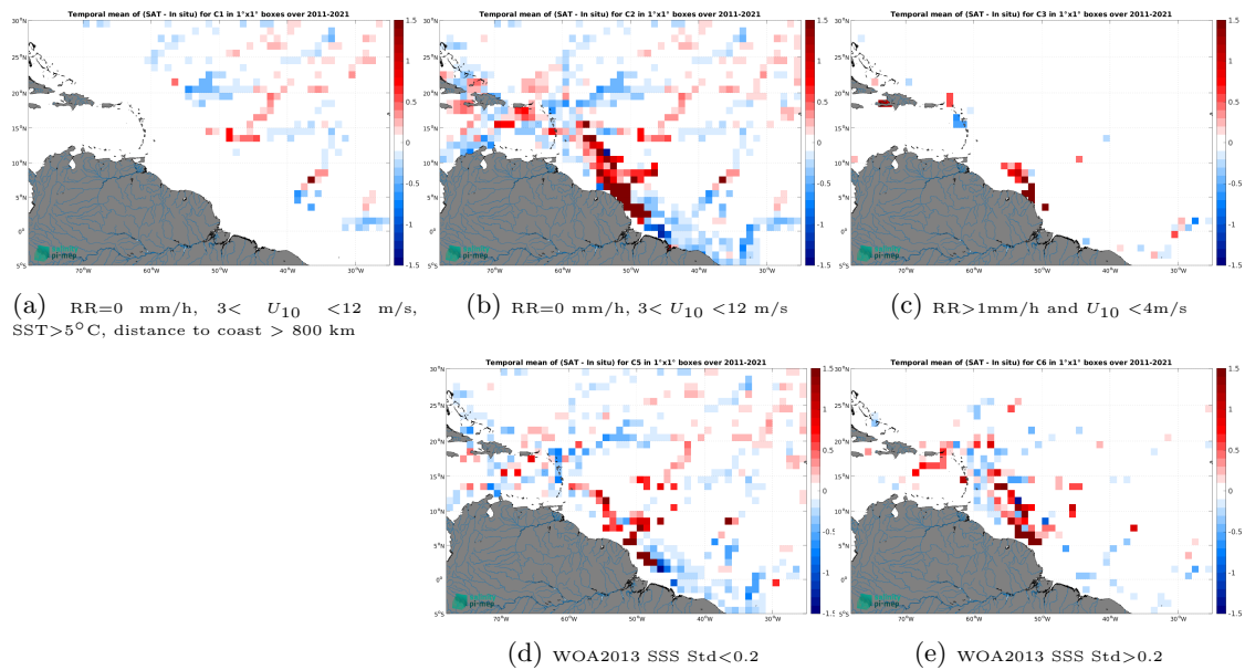
Figure 14: Temporal mean gridded over spatial boxes of size 1^\circ \times 1^\circ of \Delta SSS (SMOS SSS L4 v2 - Daily (BEC) - TSG (GOSUD-Research-vessel)) for 5 different subdatasets corresponding to:RR=0 mm/h, 3 < U_{10} < 12 m/s, SST >5^\circ\text{C} , distance to coast > 800 km (a), RR=0 mm/h, 3 < U_{10} < 12 m/s (b), RR >1 mm/h and U_{10} < 4 m/s (c), WOA2013 SSS Std <0.2 (d), WOA2013 SSS Std >0.2 (e).
