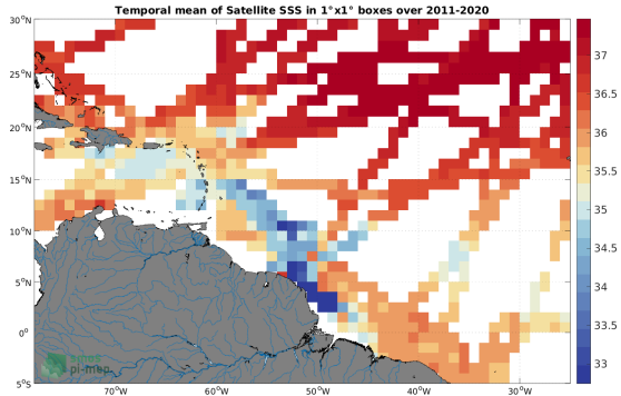
(a) MEAN(Satellite SSS)
