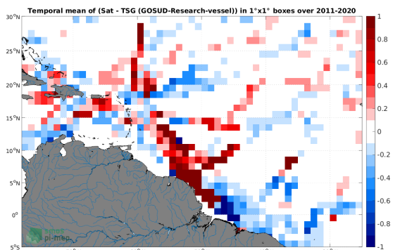
(e) MEAN( \Delta SSS) (Satellite - TSG (GOSUD-Research-vessel))
