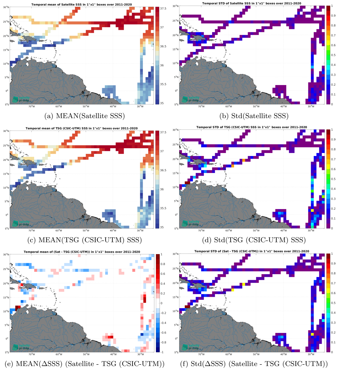
Figure 7: Temporal mean (left) and Std (right) of SSS from SMOS SSS L4 v2 - Daily (BEC) (top), TSG (CSIC-UTM) (middle), and of \Delta SSS (Satellite - TSG (CSIC-UTM)). Only match-up pairs are used to generate these maps.
