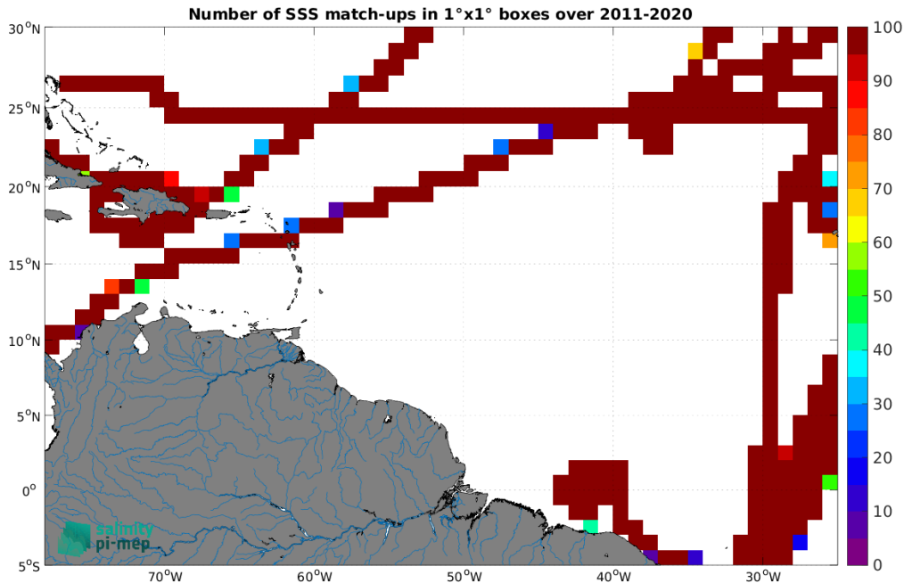
Figure 5: Number of SSS match-ups between TSG (CSIC-UTM) SSS and the SMOS SSS L4 v2 - Daily (BEC) SSS product for the Amazon and Orinoco river plumes Pi-MEP region over 1^{\circ} \times 1^{\circ} boxes and for the full satellite product period.
