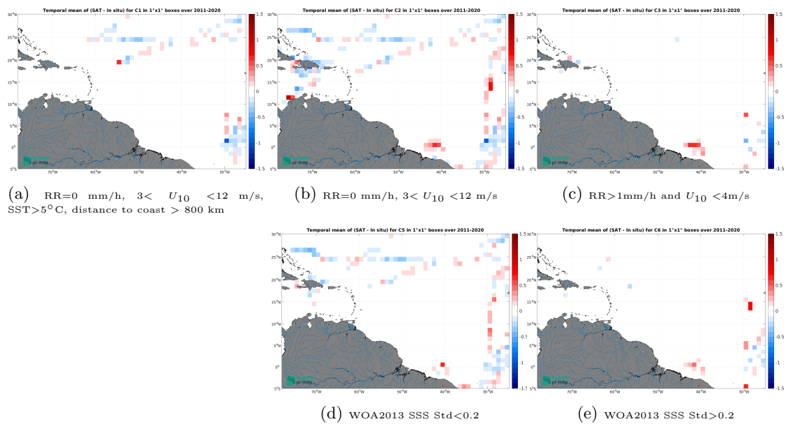
Figure 14: Temporal mean gridded over spatial boxes of size 1^\circ \times 1^\circ of \Delta SSS (SMOS SSS L4 v2 - Daily (BEC) - TSG (CSIC-UTM)) for 5 different subdatasets corresponding to:RR=0 mm/h, 3 < U_{10} < 12 m/s, SST >5^\circ\text{C} , distance to coast > 800 km (a), RR=0 mm/h, 3 < U_{10} < 12 m/s (b), RR >1 mm/h and U_{10} < 4 m/s (c), WOA2013 SSS Std <0.2 (d), WOA2013 SSS Std >0.2 (e).
