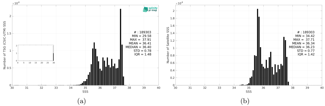
Figure 3: Histograms of SSS from TSG (CSIC-UTM) (a) and SMOS SSS L4 v2 - Daily (BEC) (b) considering all match-up pairs per bins of 0.1 over the Amazon and Orinoco river plumes Pi-MEP region and for the full satellite product period.
