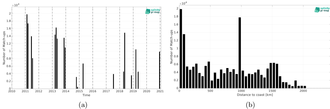
Figure 2: Number of match-ups between TSG (CSIC-UTM) and SMOS SSS L4 v2 - Daily (BEC) SSS as a function of time (a) and as function of the distance to coast (b) over the Amazon and Orinoco river plumes Pi-MEP region and for the full satellite product period.
