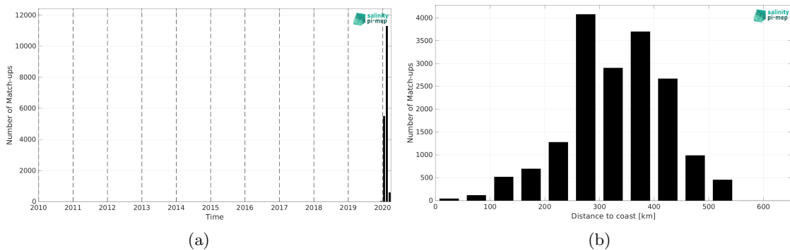
Figure 2: Number of match-ups between Saildrone and SMOS SSS L4 v2 - Daily (BEC) SSS as a function of time (a) and as function of the distance to coast (b) over the Amazon and Orinoco river plumes Pi-MEP region and for the full satellite product period.
