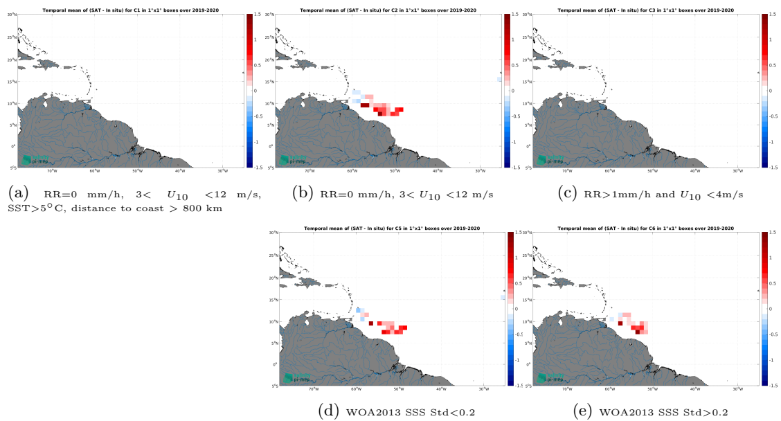
Figure 14: Temporal mean gridded over spatial boxes of size 1^\circ \times 1^\circ of \Delta\text{SSS} (SMOS SSS L4 v2 - Daily (BEC) - Sairdrone) for 5 different subdatasets corresponding to:RR=0 mm/h, 3 < U_{10} < 12 m/s, SST >5^\circ\text{C} , distance to coast > 800 km (a), RR=0 mm/h, 3 < U_{10} < 12 m/s (b), RR >1 mm/h and U_{10} < 4 m/s (c), WOA2013 SSS Std <0.2 (d), WOA2013 SSS Std >0.2 (e).
