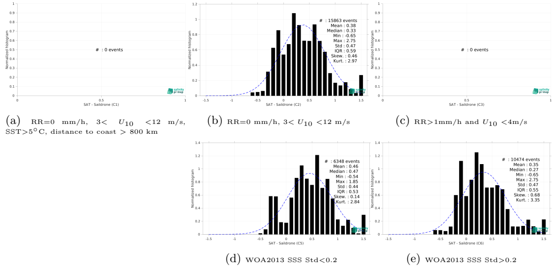
Figure 15: Normalized histogram of \Delta SSS (SMOS SSS L4 v2 - Daily (BEC) - Saildrone) for 5 different subdatasets corresponding to: RR=0 mm/h, 3 < U_{10} < 12 m/s, SST > 5°C, distance to coast > 800 km (a), RR=0 mm/h, 3 < U_{10} < 12 m/s (b), RR > 1mm/h and U_{10} < 4 m/s (c), WOA2013 SSS Std < 0.2 (d), WOA2013 SSS Std > 0.2 (e).
