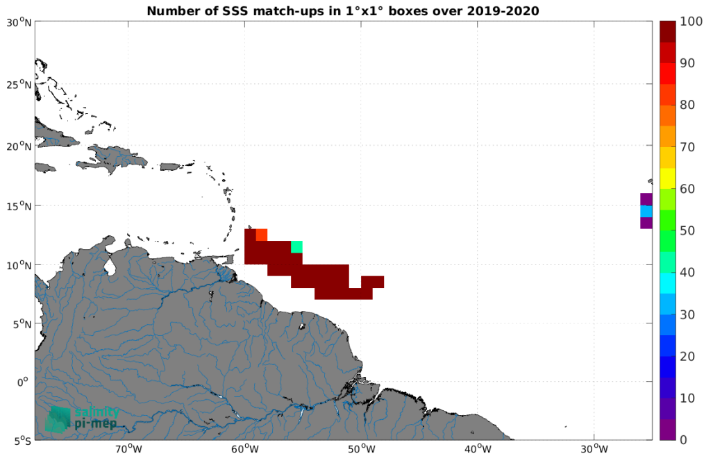
Figure 5: Number of SSS match-ups between Saildrone SSS and the SMOS SSS L4 v2 - Daily (BEC) SSS product for the Amazon and Orinoco river plumes Pi-MEP region over 1^{\circ} \times 1^{\circ} boxes and for the full satellite product period.
