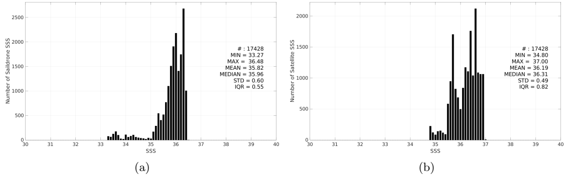
Figure 3: Histograms of SSS from Saildrone (a) and SMOS SSS L4 v2 - Daily (BEC) (b) considering all match-up pairs per bins of 0.1 over the Amazon and Orinoco river plumes Pi-MEP region and for the full satellite product period.
