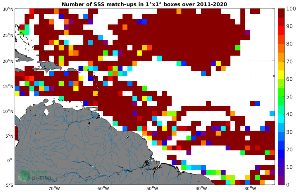
Figure 3: Number of SSS match-ups between Surface drifters SSS and the SMOS SSS L4 v2 - Daily (BEC) SSS product for the Amazon and Orinoco river plumes Pi-MEP region over 1^{\circ} \times 1^{\circ} boxes and for the full satellite product period.
