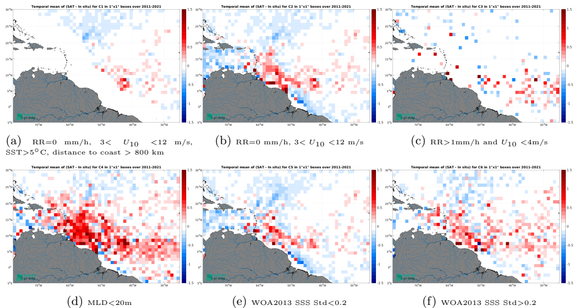
Figure 14: Temporal mean gridded over spatial boxes of size 1^\circ \times 1^\circ of \Delta SSS (SMOS SSS L4 v2 - Daily (BEC) - Argo) for 6 different subdatasets corresponding to: RR=0 mm/h, 3 < U_{10} < 12 m/s, SST > 5°C, distance to coast > 800 km (a), RR=0 mm/h, 3 < U_{10} < 12 m/s (b), RR > 1mm/h and U_{10} < 4 m/s (c), MLD < 20m (d), WOA2013 SSS Std < 0.2 (e), WOA2013 SSS Std > 0.2 (f).
