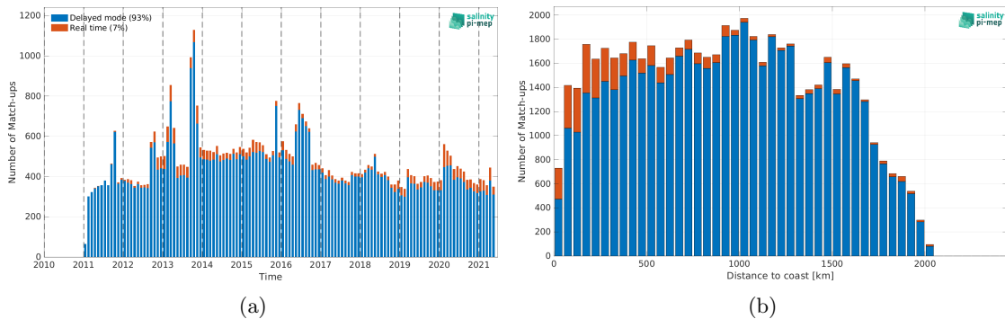
Figure 1: Number of match-ups between Argo and SMOS SSS L4 v2 - Daily (BEC) SSS as a function of time (a) and as function of the distance to coast (b) over the Amazon and Orinoco river plumes Pi-MEP region and for the full satellite product period.
