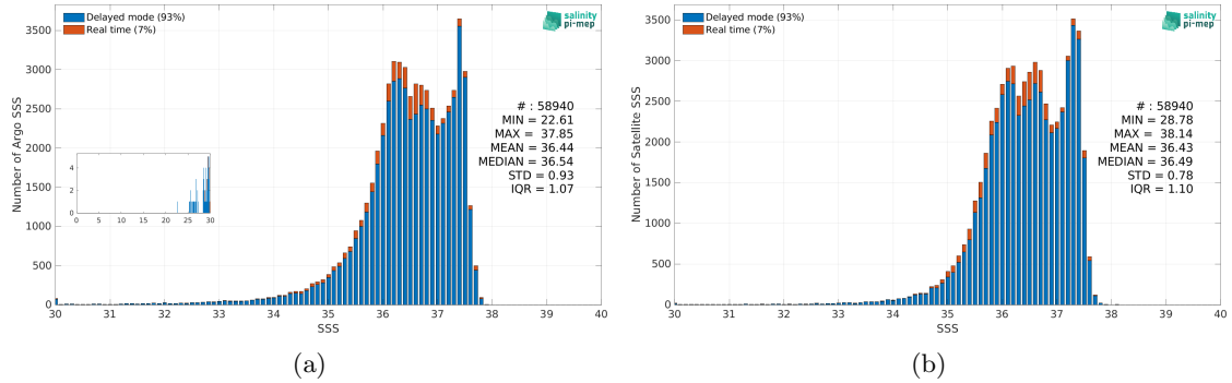
Figure 2: Histograms of SSS from Argo (a) and SMOS SSS L4 v2 - Daily (BEC) (b) considering all match-up pairs per bins of 0.1 over the Amazon and Orinoco river plumes Pi-MEP region and for the full satellite product period.
