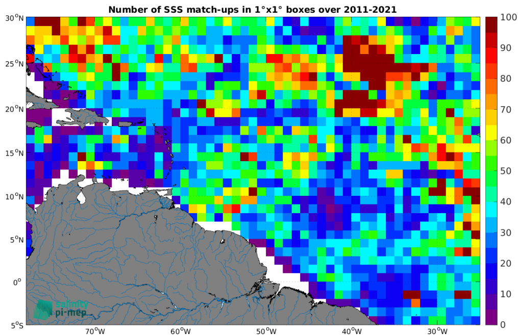
Figure 4: Number of SSS match-ups between Argo SSS and the SMOS SSS L4 v2 - Daily (BEC) SSS product for the Amazon and Orinoco river plumes Pi-MEP region over 1^\circ \times 1^\circ boxes and for the full satellite product period.
