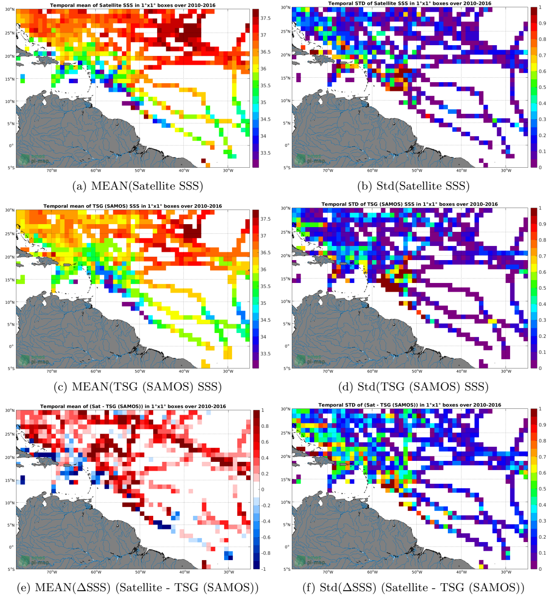
Figure 6: Temporal mean (left) and Std (right) of SSS from SMOS SSS L3 v3 Monthly (ICDC') (top), TSG (SAMOS) (middle), and of \Delta SSS (Satellite - TSG (SAMOS)). Only match-up pairs are used to generate these maps.
