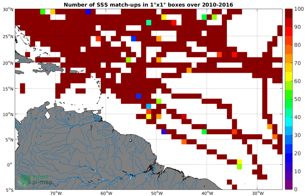
Figure 4: Number of SSS match-ups between TSG-SAMOS SSS and the SMOS-L3-ICDC-V3-MONTHLY-0.5DEG SSS product for the Amazon and Orinoco river plumes Pi-MEP region over 1°x1° boxes and for the full satellite product period.
