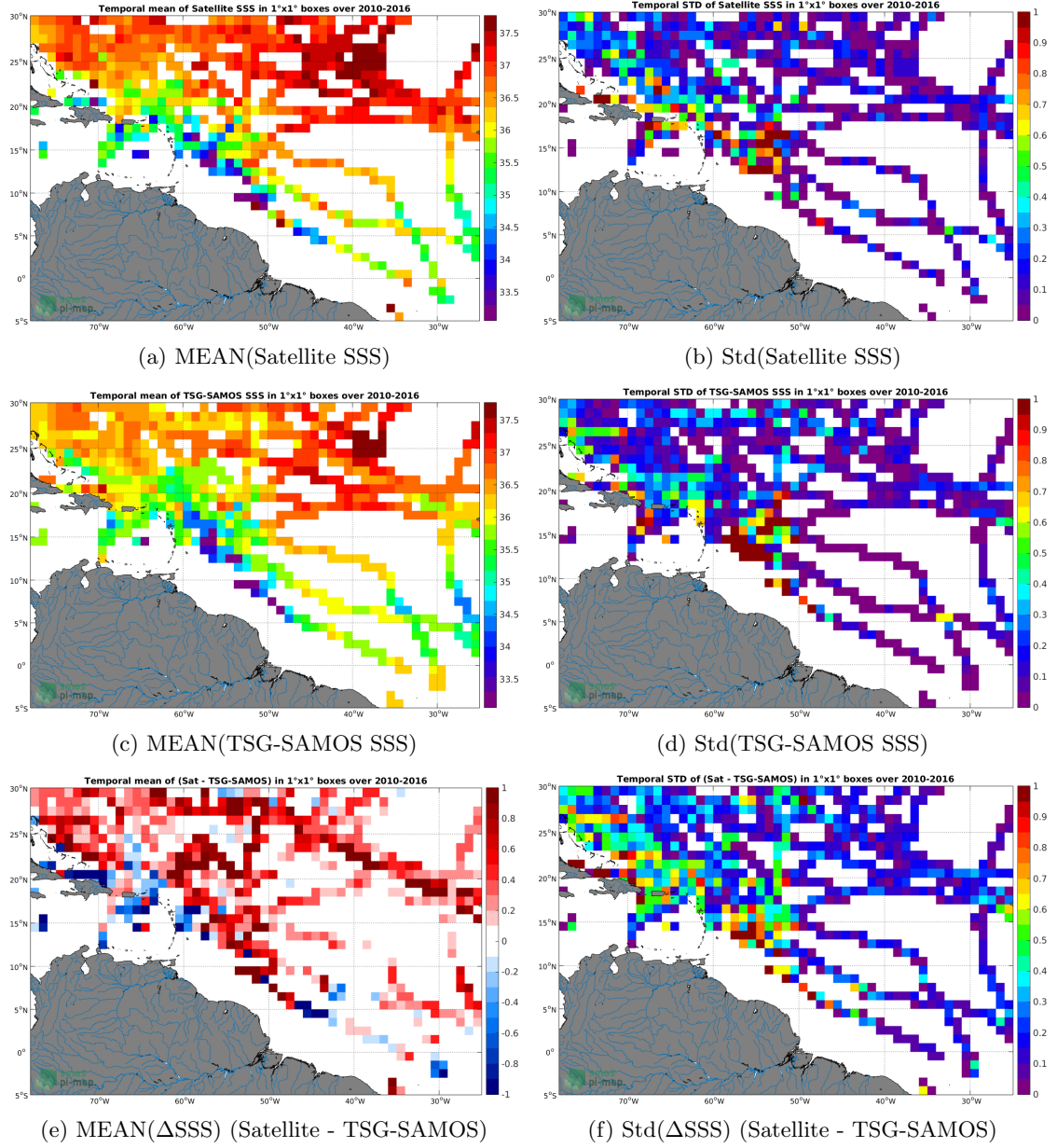
Figure 6: Temporal mean (left) and Std (right) of SSS from SMOS-L3-ICDC-V3-MONTHLY-0.5DEG (top), TSG-SAMOS (middle), and of \Delta SSS (Satellite - TSG-SAMOS). Only match-up pairs are used to generate these maps.
