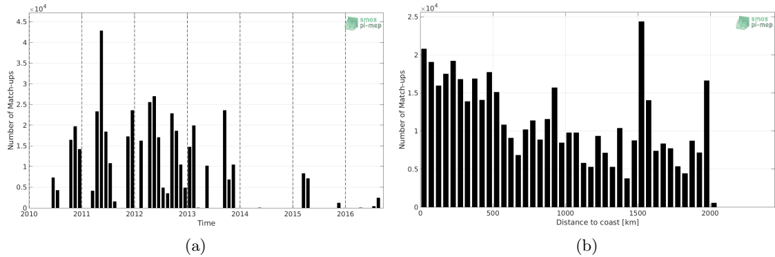
Figure 1: Number of match-ups between TSG-SAMOS and SMOS-L3-ICDC-V3-MONTHLY-0.5DEG SSS as a function of time (a) and as function of the distance to coast (b) over the Amazon and Orinoco river plumes Pi-MEP region and for the full satellite product period.
