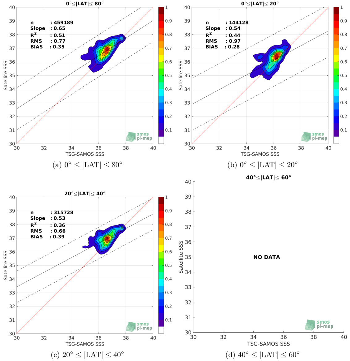
Figure 9: Contour maps of the concentration of SMOS-L3-ICDC-V3-MONTHLY-0.5DEG SSS (y-axis) versus TSG-SAMOS SSS (x-axis) at match-up pairs for different latitude bands. For each plot, the red line shows x=y . The black thin and dashed lines indicate a linear fit through the data cloud and the \pm 95\% confidence levels, respectively. The number match-up pairs n , the slope and R^2 coefficient of the linear fit, the root mean square (RMS) and the mean bias between satellite and in situ data are indicated for each latitude band in each plots.
