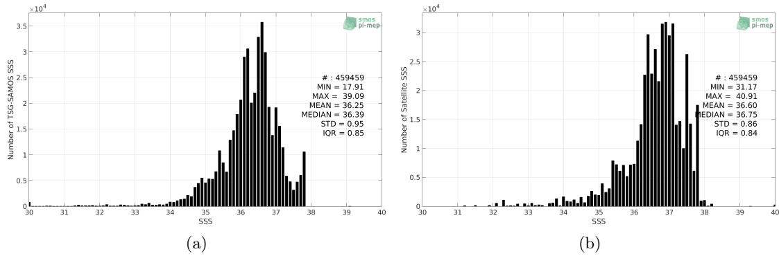
Figure 2: Histograms of SSS from TSG-SAMOS (a) and SMOS-L3-ICDC-V3-MONTHLY-0.5DEG (b) considering all match-up pairs per bins of 0.1 over the Amazon and Orinoco river plumes Pi-MEP region and for the full satellite product period.
