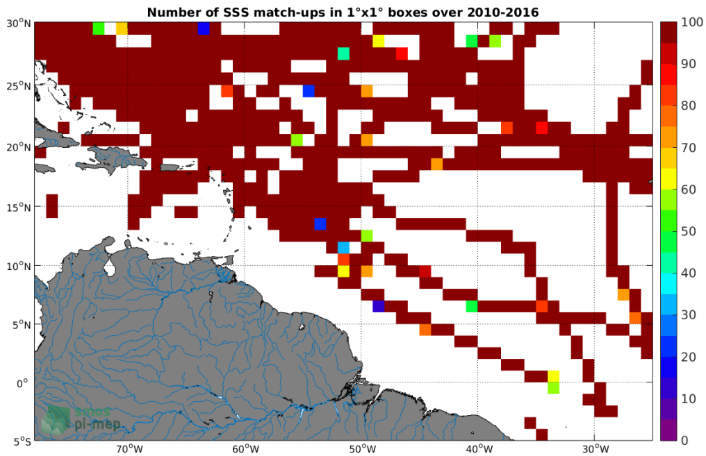
Figure 4: Number of SSS match-ups between TSG-SAMOS SSS and the SMOS-L3-ICDC-V3-MONTHLY-0.5DEG SSS product for the Amazon and Orinoco river plumes Pi-MEP region over 1^\circ \times 1^\circ boxes and for the full satellite product period.
