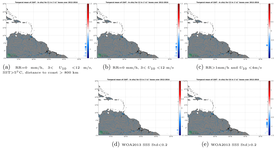
Figure 12: Temporal mean gridded over spatial boxes of size 1^\circ \times 1^\circ of \Delta SSS (SMOS SSS L3 v3 Monthly (ICDC) - TSG (Polarstern)) for 5 different subdatasets corresponding to:RR=0 mm/h, 3 < U_{10} < 12 m/s, SST >5^\circ\text{C} , distance to coast > 800 km (a), RR=0 mm/h, 3 < U_{10} < 12 m/s (b), RR >1 mm/h and U_{10} < 4 m/s (c), WOA2013 SSS Std <0.2 (d), WOA2013 SSS Std >0.2 (e).
