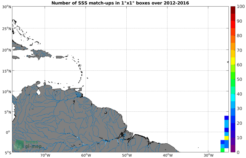
Figure 4: Number of SSS match-ups between TSG (Polarstern) SSS and the SMOS SSS L3 v3 Monthly (ICDC) SSS product for the Amazon and Orinoco river plumes Pi-MEP region over 1^\circ \times 1^\circ boxes and for the full satellite product period.
