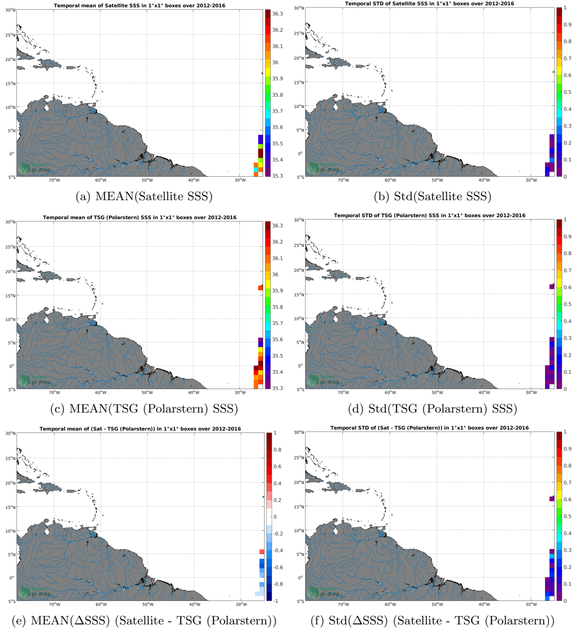
Figure 6: Temporal mean (left) and Std (right) of SSS from SMOS SSS L3 v3 Monthly (ICDC) (top), TSG (Polarstern) (middle), and of \Delta SSS (Satellite - TSG (Polarstern)). Only match-up pairs are used to generate these maps.
