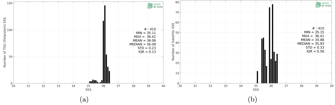
Figure 2: Histograms of SSS from TSG (Polarstern) (a) and SMOS SSS L3 v3 Monthly (ICDC) (b) considering all match-up pairs per bins of 0.1 over the Amazon and Orinoco river plumes Pi-MEP region and for the full satellite product period.
