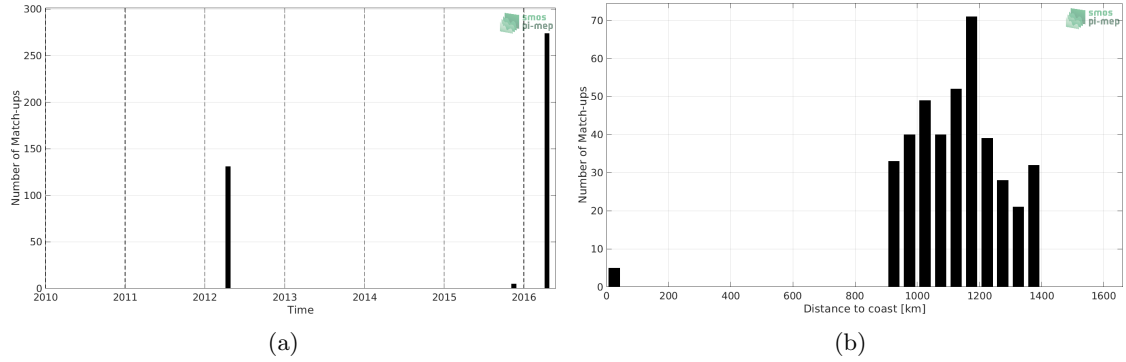
Figure 1: Number of match-ups between TSG (Polarstern) and SMOS SSS L3 v3 Monthly (ICDC) SSS as a function of time (a) and as function of the distance to coast (b) over the Amazon and Orinoco river plumes Pi-MEP region and for the full satellite product period.
