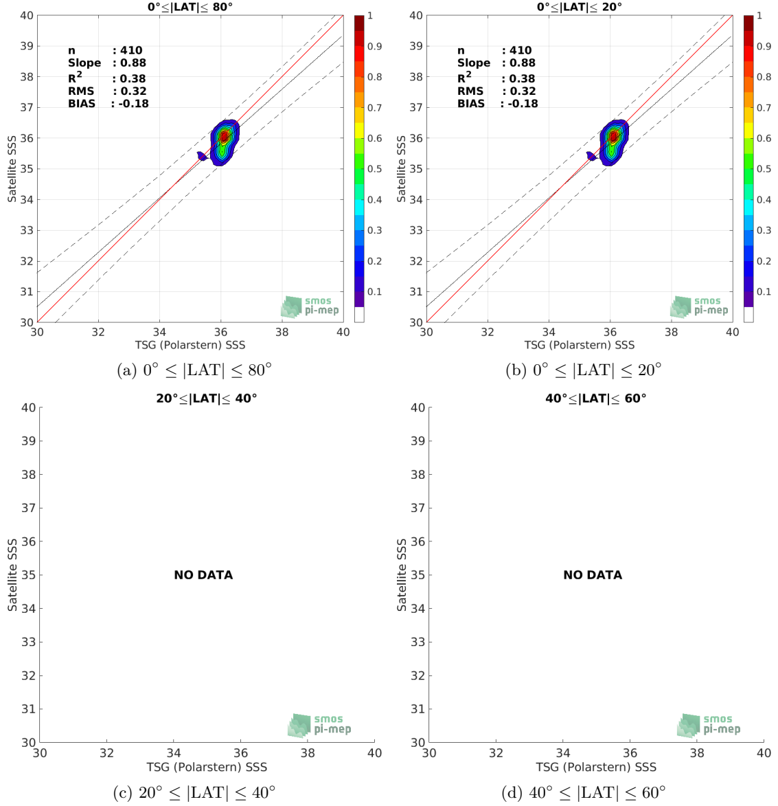
Figure 9: Contour maps of the concentration of SMOS SSS L3 v3 Monthly (ICDC) SSS (y-axis) versus TSG (Polarstern) SSS (x-axis) at match-up pairs for different latitude bands. For each plot, the red line shows x=y . The black thin and dashed lines indicate a linear fit through the data cloud and the \pm 95\% confidence levels, respectively. The number match-up pairs n , the slope and R^2 coefficient of the linear fit, the root mean square (RMS) and the mean bias between satellite and in situ data are indicated for each latitude band in each plots.
