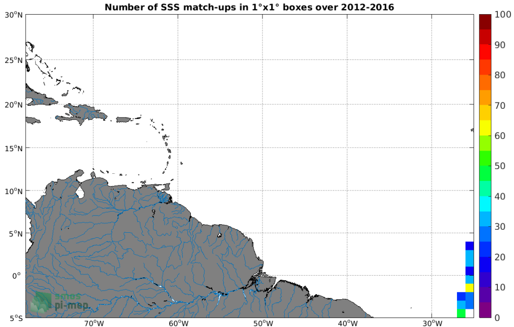
Figure 4: Number of SSS match-ups between TSG (Polarstern) SSS and the SMOS SSS L3 v3 Monthly (ICDC) SSS product for the Amazon and Orinoco river plumes Pi-MEP region over 1°x1° boxes and for the full satellite product period.
