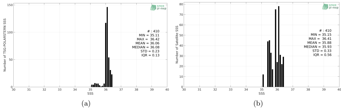
Figure 2: Histograms of SSS from TSG-POLARSTERN (a) and SMOS-L3-ICDC-V3-MONTHLY-0.5DEG (b) considering all match-up pairs per bins of 0.1 over the Amazon and Orinoco river plumes Pi-MEP region and for the full satellite product period.
