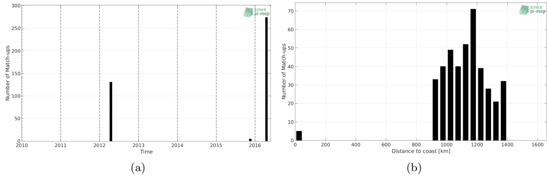
Figure 1: Number of match-ups between TSG-POLARSTERN and SMOS-L3-ICDC-V3-MONTHLY-0.5DEG SSS as a function of time (a) and as function of the distance to coast (b) over the Amazon and Orinoco river plumes Pi-MEP region and for the full satellite product period.
