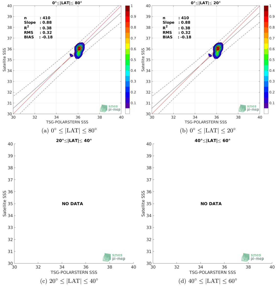
Figure 9: Contour maps of the concentration of SMOS-L3-ICDC-V3-MONTHLY-0.5DEG SSS (y-axis) versus TSG-POLARSTERN SSS (x-axis) at match-up pairs for different latitude bands. For each plot, the red line shows x=y . The black thin and dashed lines indicate a linear fit through the data cloud and the \pm 95\% confidence levels, respectively. The number match-up pairs n , the slope and R^2 coefficient of the linear fit, the root mean square (RMS) and the mean bias between satellite and in situ data are indicated for each latitude band in each plots.
