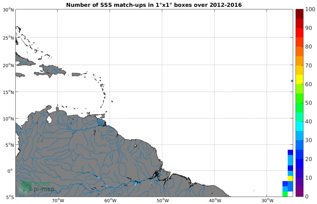
Figure 4: Number of SSS match-ups between TSG-POLARSTERN SSS and the SMOS-L3-ICDC-V3-MONTHLY-0.5DEG SSS product for the Amazon and Orinoco river plumes Pi-MEP region over 1^\circ \times 1^\circ boxes and for the full satellite product period.
