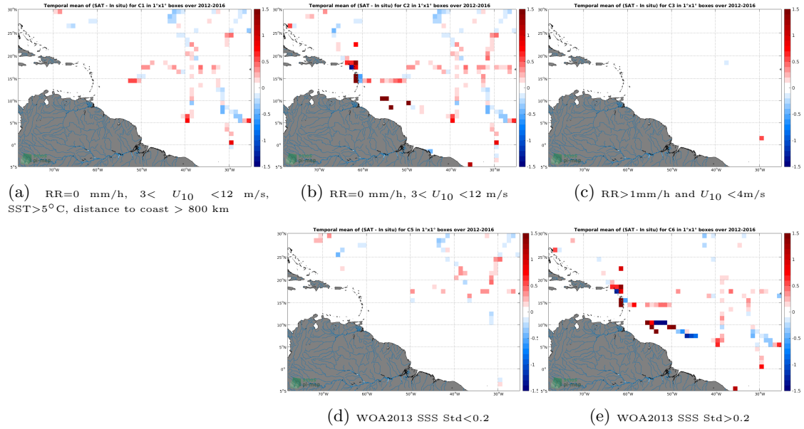
Figure 12: Temporal mean gridded over spatial boxes of size 1^\circ \times 1^\circ of \Delta SSS (SMOS SSS L3 v3 Monthly (ICDC) - TSG (GOSUD-Sailing-ship)) for 5 different subdatasets corresponding to: RR=0 mm/h, 3 < U_{10} < 12 m/s, SST > 5^\circ C , distance to coast > 800 km (a), RR=0 mm/h, 3 < U_{10} < 12 m/s (b), RR > 1 mm/h and U_{10} < 4 m/s (c), WOA2013 SSS Std < 0.2 (d), WOA2013 SSS Std > 0.2 (e).
