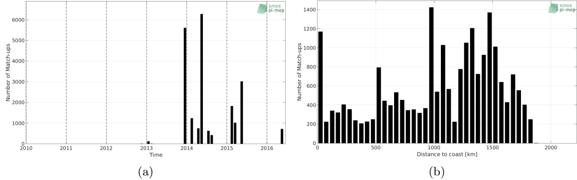
Figure 1: Number of match-ups between TSG (GOSUD-Sailing-ship) and SMOS SSS L3 v3 Monthly (ICDC) SSS as a function of time (a) and as function of the distance to coast (b) over the Amazon and Orinoco river plumes Pi-MEP region and for the full satellite product period.
