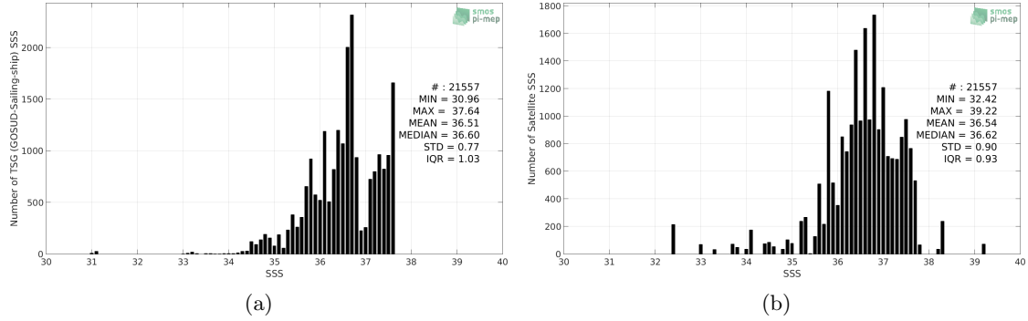
Figure 2: Histograms of SSS from TSG (GOSUD-Sailing-ship) (a) and SMOS SSS L3 v3 Monthly (ICDC) (b) considering all match-up pairs per bins of 0.1 over the Amazon and Orinoco river plumes Pi-MEP region and for the full satellite product period.
