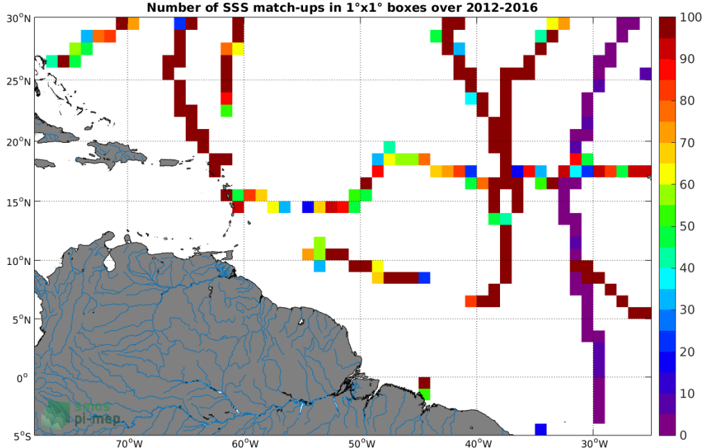
Figure 4: Number of SSS match-ups between TSG (GOSUD-Sailing-ship) SSS and the SMOS SSS L3 v3 Monthly (ICDC) SSS product for the Amazon and Orinoco river plumes Pi-MEP region over 1^\circ \times 1^\circ boxes and for the full satellite product period.
