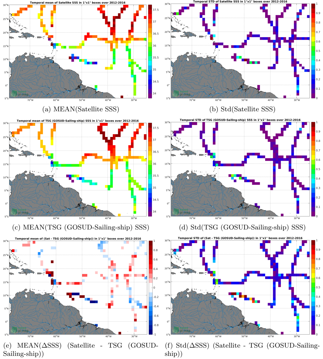
Figure 6: Temporal mean (left) and Std (right) of SSS from SMOS SSS L3 v3 Monthly (ICDC') (top), TSG (GOSUD-Sailing-ship) (middle), and of \Delta SSS (Satellite - TSG (GOSUD-Sailing-ship)). Only match-up pairs are used to generate these maps.
