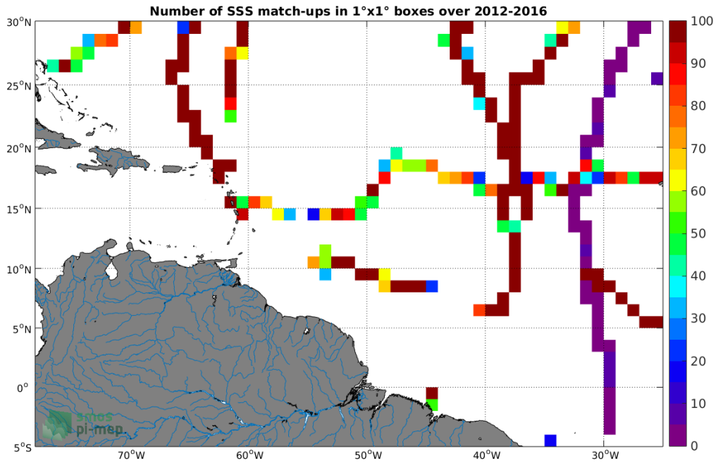
Figure 4: Number of SSS match-ups between TSG-GOSUD-Sailing-ship SSS and the SMOS-L3-ICDC-V3-MONTHLY-0.5DEG SSS product for the Amazon and Orinoco river plumes Pi-MEP region over 1°x1° boxes and for the full satellite product period.
