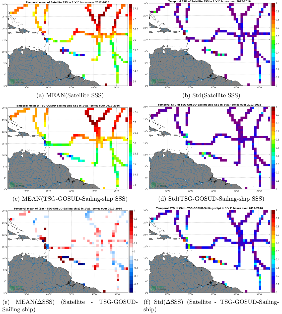
Figure 6: Temporal mean (left) and Std (right) of SSS from SMOS-L3-ICDC-V3-MONTHLY-0.5DEG (top), TSG-GOSUD-Sailing-ship (middle), and of \Delta SSS (Satellite - TSG-GOSUD-Sailing-ship). Only match-up pairs are used to generate these maps.
