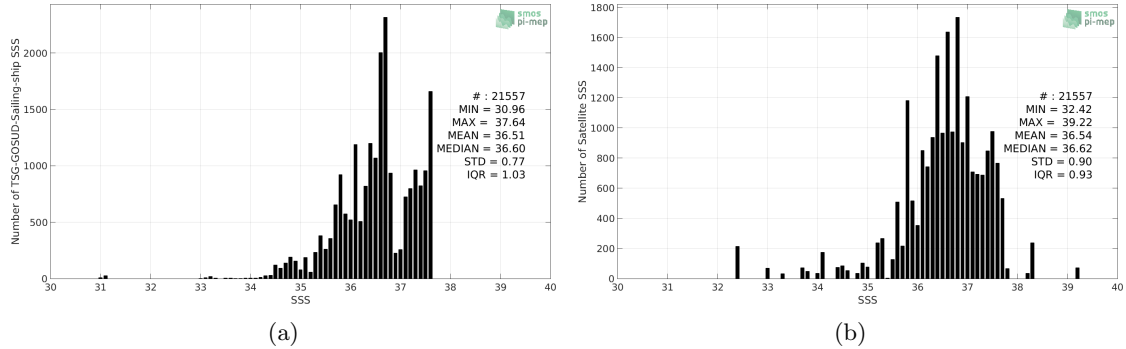
Figure 2: Histograms of SSS from TSG-GOSUD-Sailing-ship (a) and SMOS-L3-ICDC-V3-MONTHLY-0.5DEG (b) considering all match-up pairs per bins of 0.1 over the Amazon and Orinoco river plumes Pi-MEP region and for the full satellite product period.
