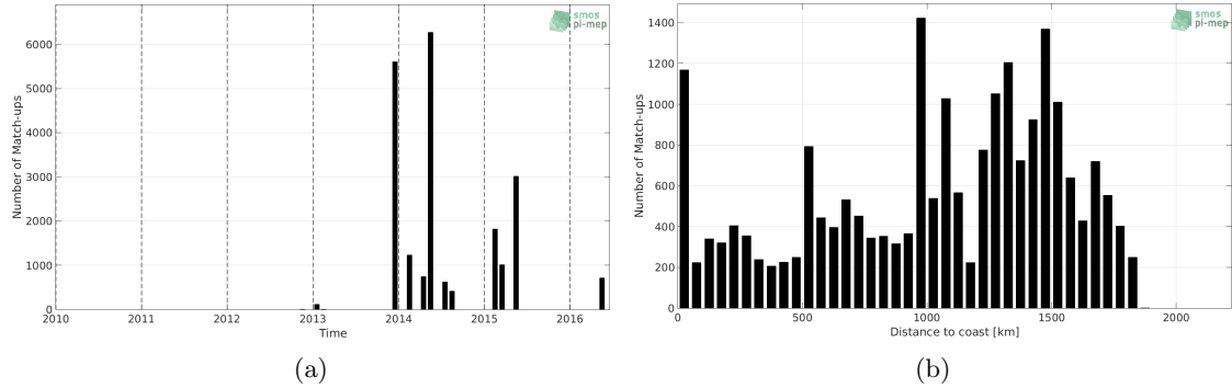
Figure 1: Number of match-ups between TSG-GOSUD-Sailing-ship and SMOS-L3-ICDC-V3-MONTHLY-0.5DEG SSS as a function of time (a) and as function of the distance to coast (b) over the Amazon and Orinoco river plumes Pi-MEP region and for the full satellite product period.
