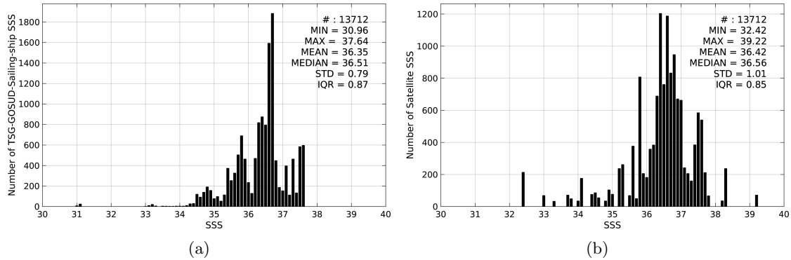
Figure 2: Histograms of SSS from TSG-GOSUD-Sailing-ship (a) and SMOS-L3-ICDC-V3-MONTHLY-0.5DEG (b) considering all match-up pairs per bins of 0.1 over the Amazon and Orinoco river plumes Pi-MEP region and for the full satellite product period.
