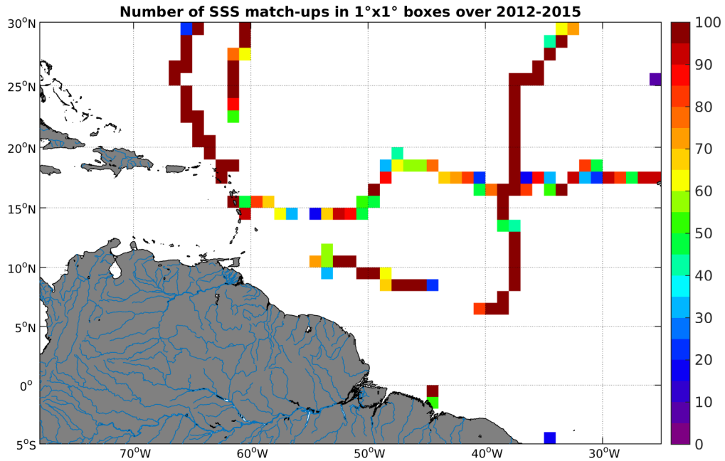
Figure 4: Number of SSS match-ups between TSG-GOSUD-Sailing-ship SSS and the SMOS-L3-ICDC-V3-MONTHLY-0.5DEG SSS product for the Amazon and Orinoco river plumes Pi-MEP region over 1^\circ \times 1^\circ boxes and for the full satellite product period.
