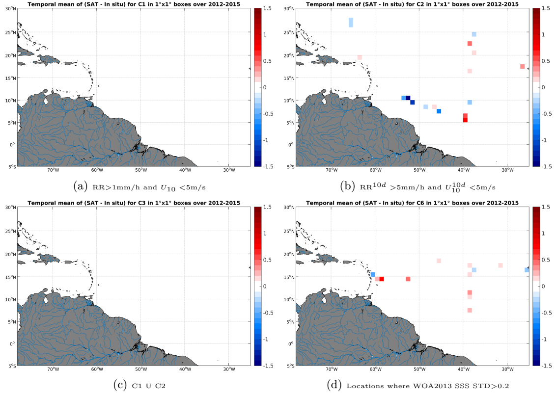
Figure 12: Temporal mean gridded over spatial boxes of size 1^\circ \times 1^\circ of \Delta SSS (SMOS-L3-ICDC-V3-MONTHLY-0.5DEG - TSG-GOSUD-Sailing-ship) for 4 different subdatasets corresponding to: RR > 1mm/h and U_{10} < 5 m/s (a), RR^{10d} > 5 mm/h and U_{10}^{10d} < 5 m/s (b), C1 U C2 (c), Locations where WOA2013 SSS STD > 0.2 (d).
