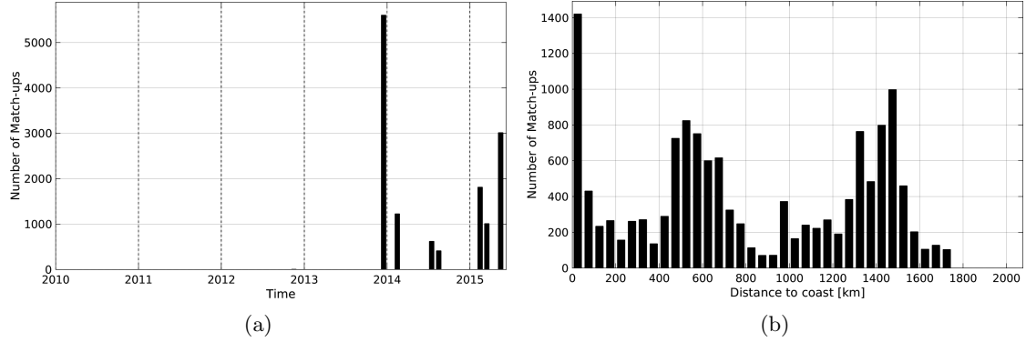
Figure 1: Number of match-ups between TSG-GOSUD-Sailing-ship and SMOS-L3-ICDC-V3-MONTHLY-0.5DEG SSS as a function of time (a) and as function of the distance to coast (b) over the Amazon and Orinoco river plumes Pi-MEP region and for the full satellite product period.
