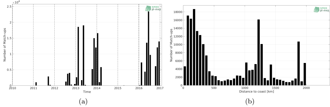
Figure 1: Number of match-ups between TSG (GOSUD-Research-vessel) and SMOS SSS L3 v3 Monthly (ICDC) SSS as a function of time (a) and as function of the distance to coast (b) over the Amazon and Orinoco river plumes Pi-MEP region and for the full satellite product period.
