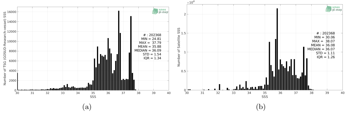
Figure 2: Histograms of SSS from TSG (GOSUD-Research-vessel) (a) and SMOS SSS L3 v3 Monthly (ICDC) (b) considering all match-up pairs per bins of 0.1 over the Amazon and Orinoco river plumes Pi-MEP region and for the full satellite product period.
