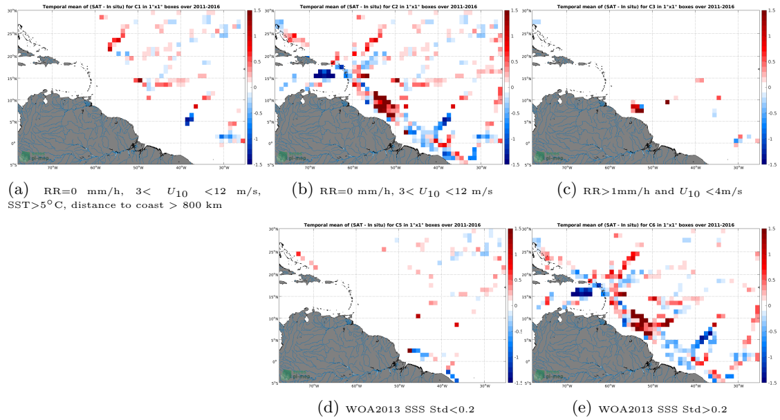
Figure 12: Temporal mean gridded over spatial boxes of size 1^\circ \times 1^\circ of \Delta SSS (SMOS SSS L3 v3 Monthly (ICDC) - TSG (GOSUD-Research-vessel)) for 5 different subdatasets corresponding to: RR=0 mm/h, 3 < U_{10} < 12 m/s, SST > 5^\circ C , distance to coast > 800 km (a), RR=0 mm/h, 3 < U_{10} < 12 m/s (b), RR > 1 mm/h and U_{10} < 4 m/s (c), WOA2013 SSS Std < 0.2 (d), WOA2013 SSS Std > 0.2 (e).
