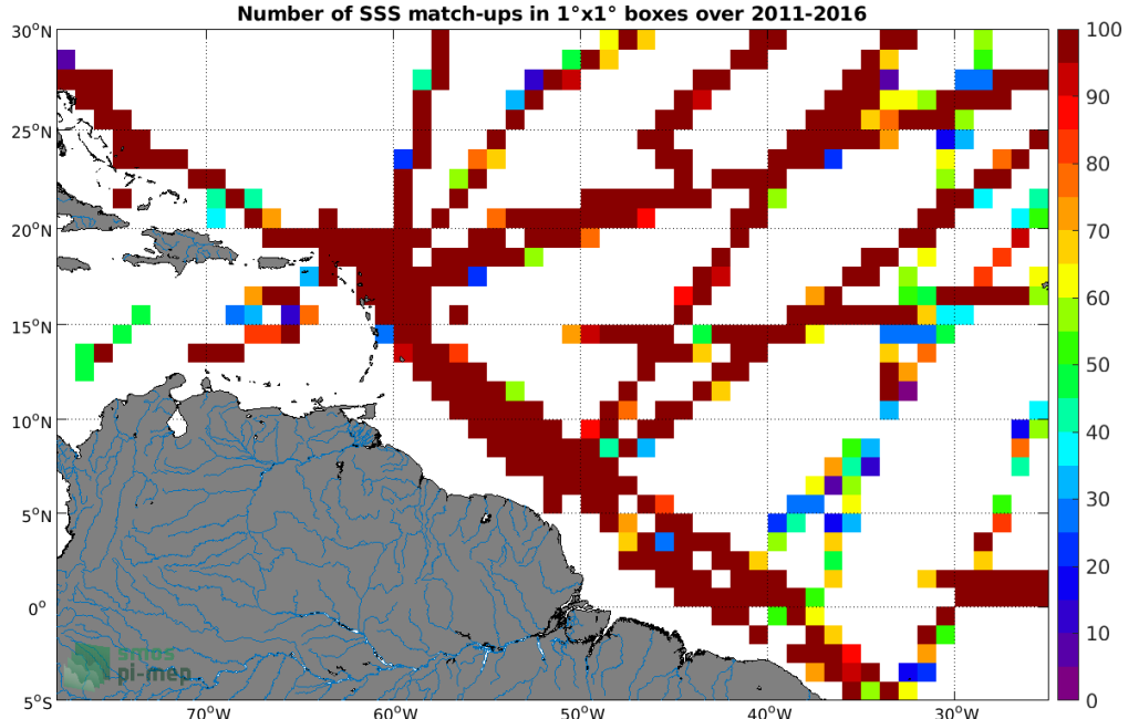
Figure 4: Number of SSS match-ups between TSG (GOSUD-Research-vessel) SSS and the SMOS SSS L3 v3 Monthly (ICDC) SSS product for the Amazon and Orinoco river plumes Pi-MEP region over 1^\circ \times 1^\circ boxes and for the full satellite product period.
