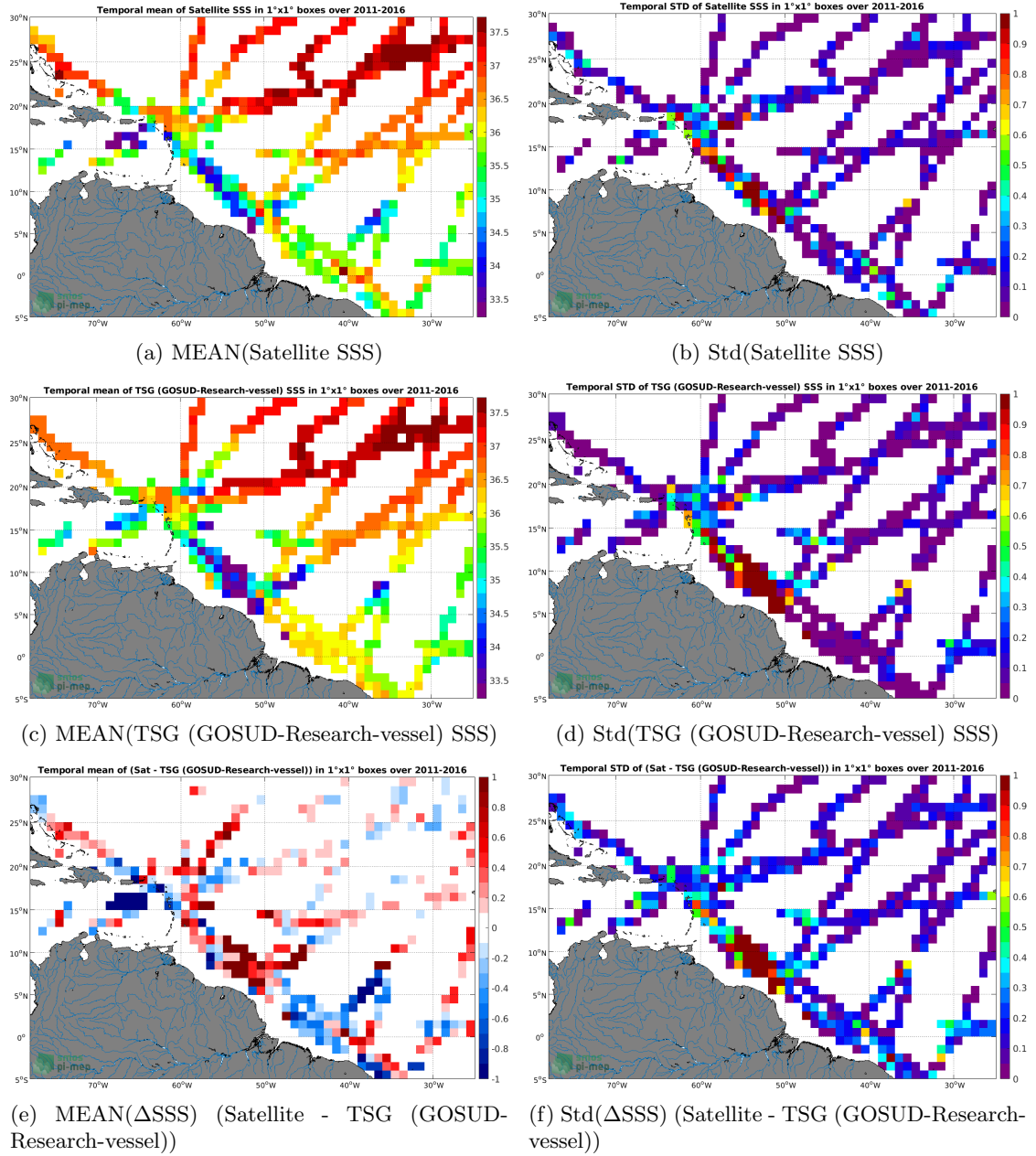
Figure 6: Temporal mean (left) and Std (right) of SSS from SMOS SSS L3 v3 Monthly (ICDC) (top), TSG (GOSUD-Research-vessel) (middle), and of \Delta SSS (Satellite - TSG (GOSUD-Research-vessel)). Only match-up pairs are used to generate these maps.
