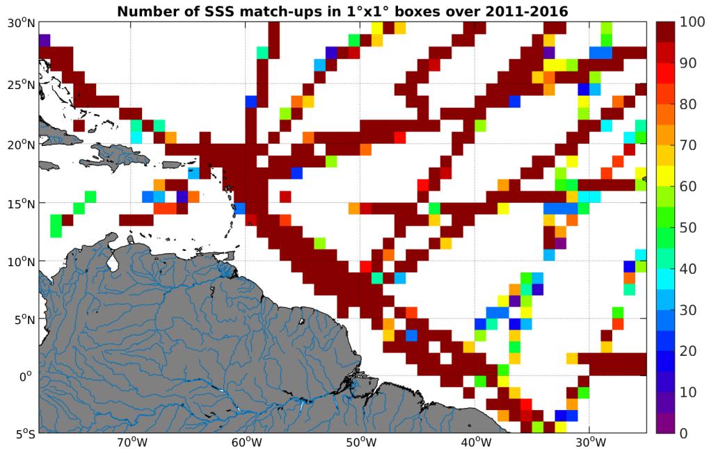
Figure 4: Number of SSS match-ups between TSG-GOSUD-Research-vessel SSS and the SMOS-L3-ICDC-V3-MONTHLY-0.5DEG SSS product for the Amazon and Orinoco river plumes Pi-MEP region over 1^\circ \times 1^\circ boxes and for the full satellite product period.
