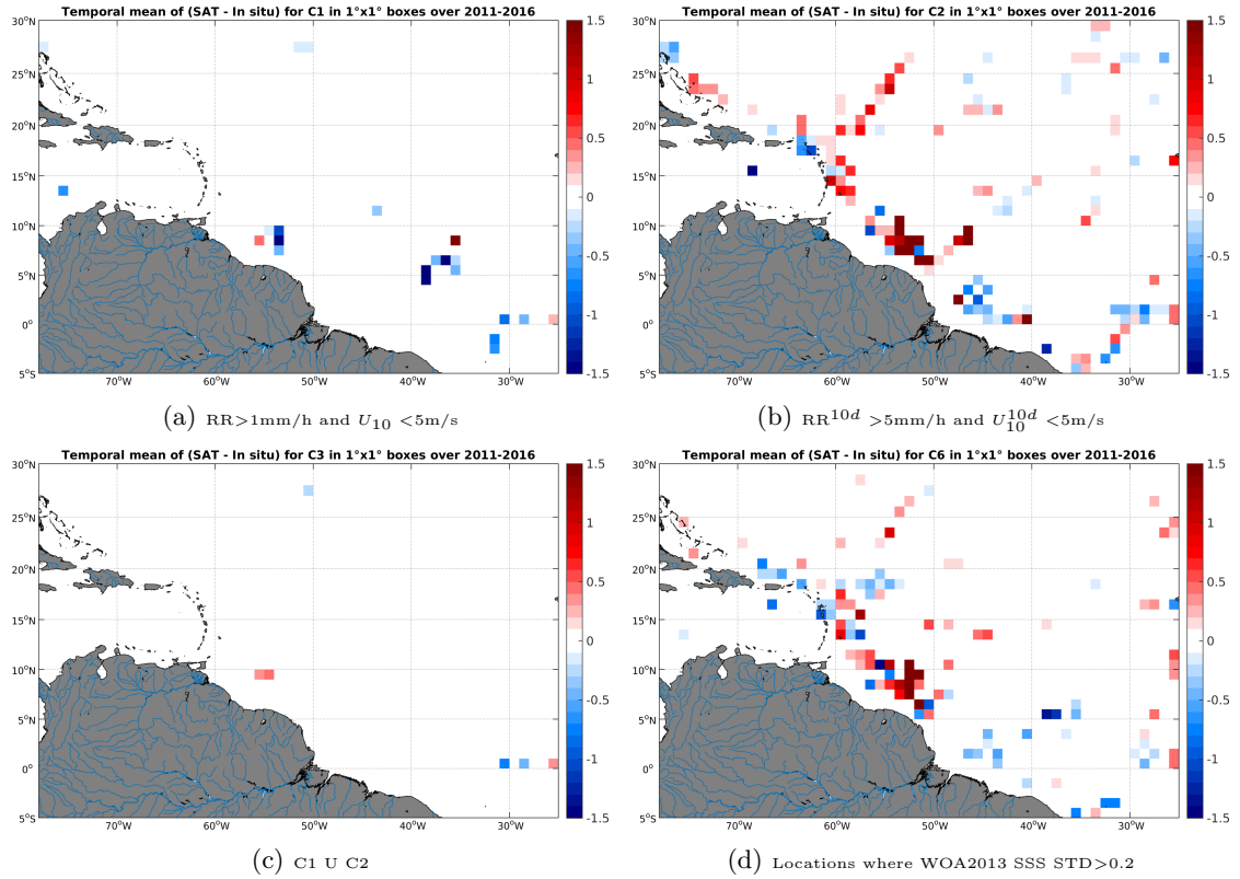
Figure 12: Temporal mean gridded over spatial boxes of size 1^\circ \times 1^\circ of \Delta SSS (SMOS-L3-ICDC-V3-MONTHLY-0.5DEG - TSG-GOSUD-Research-vessel) for 4 different subdatasets corresponding to: RR > 1mm/h and U_{10} < 5 m/s (a), RR^{10d} > 5 mm/h and U_{10}^{10d} < 5 m/s (b), C1 U C2 (c), Locations where WOA2013 SSS STD > 0.2 (d).
