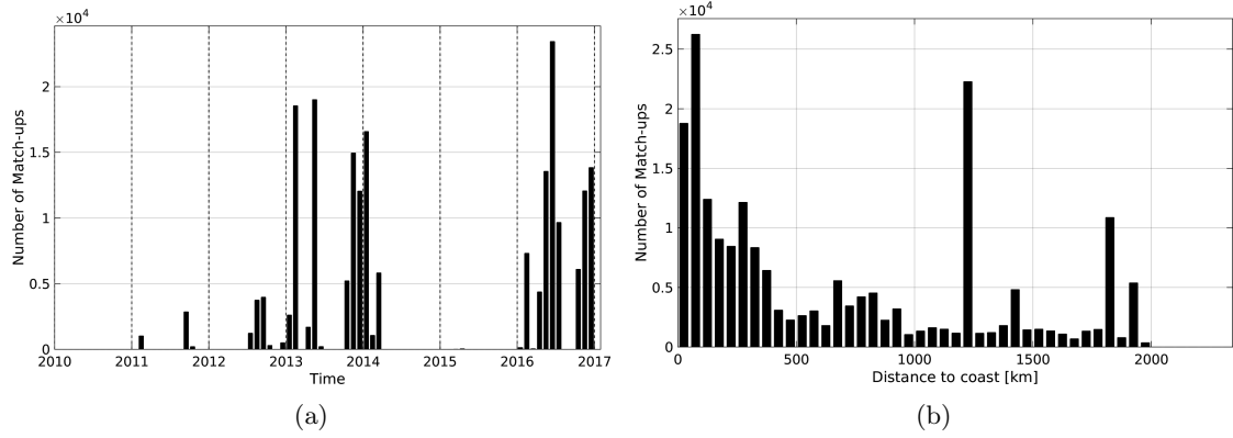
Figure 1: Number of match-ups between TSG-GOSUD-Research-vessel and SMOS-L3-ICDC-V3-MONTHLY-0.5DEG SSS as a function of time (a) and as function of the distance to coast (b) over the Amazon and Orinoco river plumes Pi-MEP region and for the full satellite product period.
