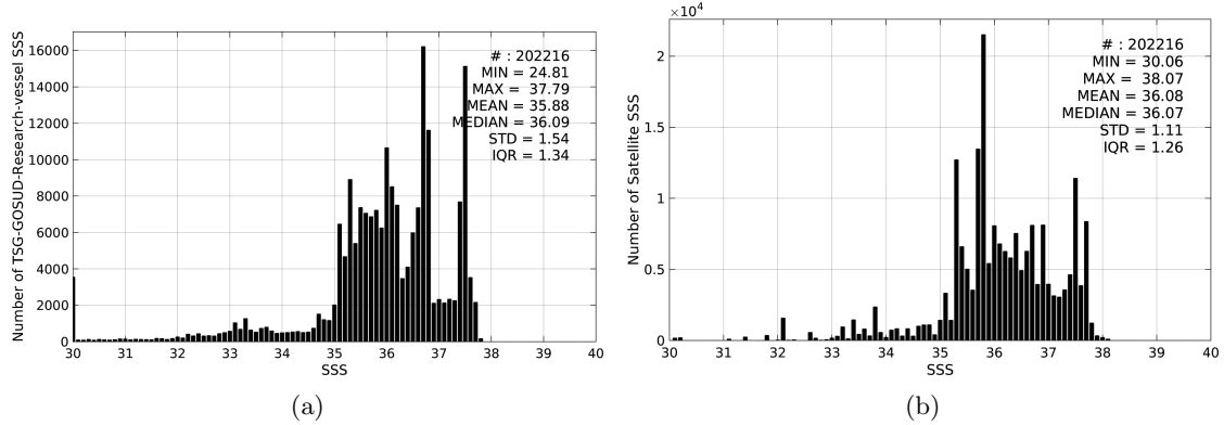
Figure 2: Histograms of SSS from TSG-GOSUD-Research-vessel (a) and SMOS-L3-ICDC-V3-MONTHLY-0.5DEG (b) considering all match-up pairs per bins of 0.1 over the Amazon and Orinoco river plumes Pi-MEP region and for the full satellite product period.
