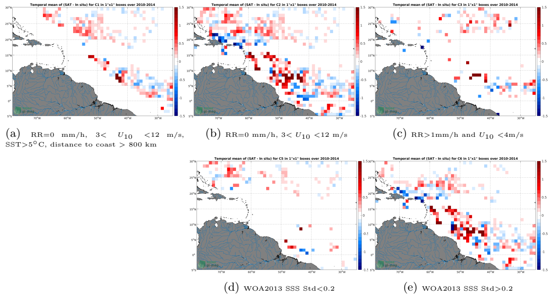
Figure 11: Temporal mean gridded over spatial boxes of size 1^\circ \times 1^\circ of \Delta SSS (SMOS SSS L3 v3 Monthly (ICDC) - Surface drifters) for 5 different subdatasets corresponding to:RR=0 mm/h, 3 < U_{10} < 12 m/s, SST >5^\circ\text{C} , distance to coast > 800 km (a), RR=0 mm/h, 3 < U_{10} < 12 m/s (b), RR >1 mm/h and U_{10} < 4 m/s (c), WOA2013 SSS Std <0.2 (d), WOA2013 SSS Std >0.2 (e).
