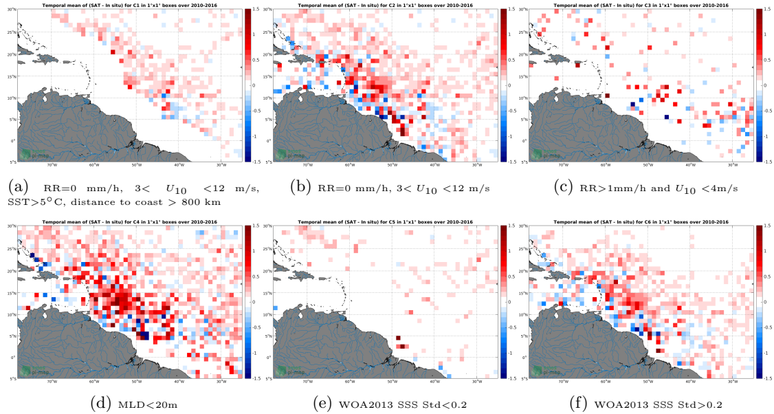
Figure 12: Temporal mean gridded over spatial boxes of size 1^\circ \times 1^\circ of \Delta SSS (SMOS SSS L3 v3 Monthly (ICDC) - Argo) for 6 different subdatasets corresponding to: RR=0 mm/h, 3 < U_{10} < 12 m/s, SST > 5^\circ C , distance to coast > 800 km (a), RR=0 mm/h, 3 < U_{10} < 12 m/s (b), RR > 1 mm/h and U_{10} < 4 m/s (c), MLD < 20 m (d), WOA2013 SSS Std < 0.2 (e), WOA2013 SSS Std > 0.2 (f).
