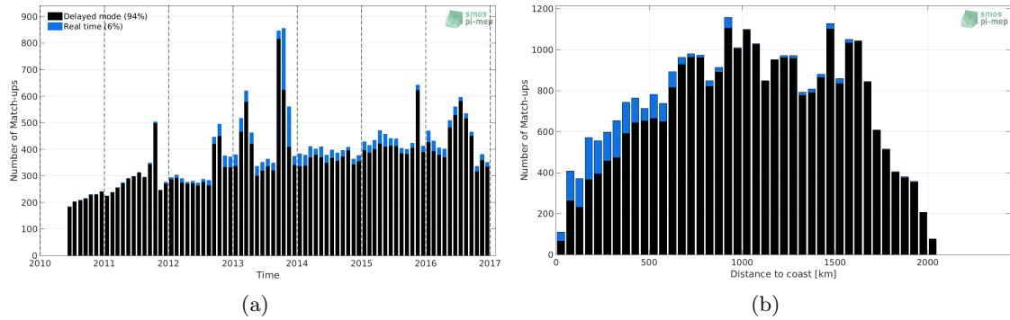
Figure 1: Number of match-ups between Argo and SMOS SSS L3 v3 Monthly (ICDC) SSS as a function of time (a) and as function of the distance to coast (b) over the Amazon and Orinoco river plumes Pi-MEP region and for the full satellite product period.
