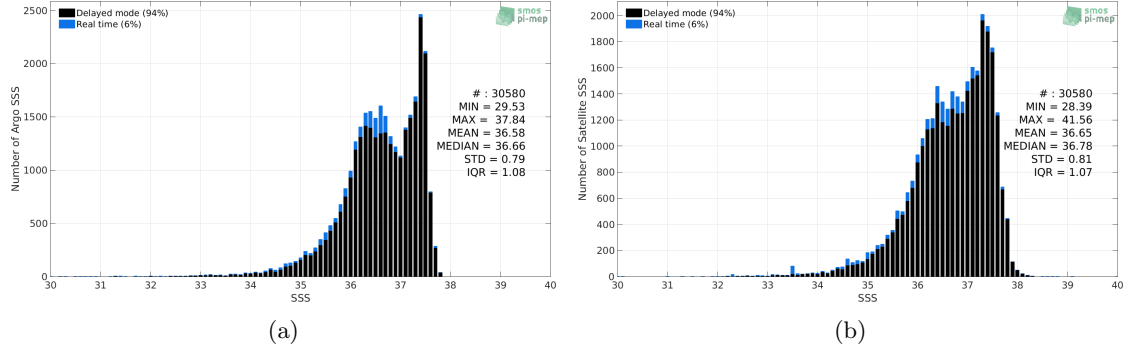
Figure 2: Histograms of SSS from Argo (a) and SMOS SSS L3 v3 Monthly (ICDC) (b) considering all match-up pairs per bins of 0.1 over the Amazon and Orinoco river plumes Pi-MEP region and for the full satellite product period.
