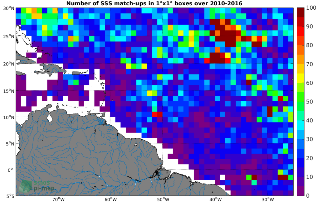
Figure 4: Number of SSS match-ups between Argo SSS and the SMOS SSS L3 v3 Monthly (ICDC) SSS product for the Amazon and Orinoco river plumes Pi-MEP region over 1^\circ \times 1^\circ boxes and for the full satellite product period.
