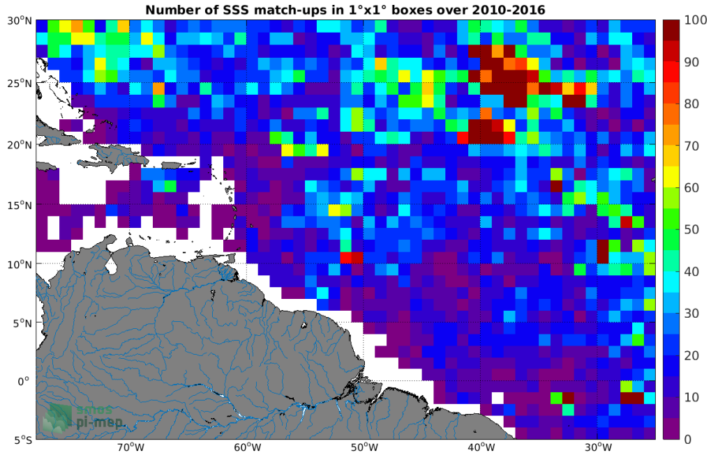
Figure 4: Number of SSS match-ups between Argo SSS and the SMOS SSS L3 v3 Monthly (ICDC) SSS product for the Amazon and Orinoco river plumes Pi-MEP region over 1°x1° boxes and for the full satellite product period.
