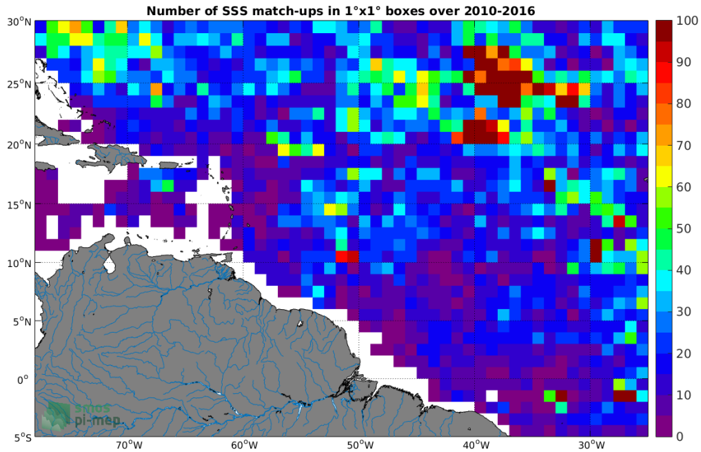
Figure 4: Number of SSS match-ups between Argos SSS and the SMOS-L3-ICDC-V3-MONTHLY-0.5DEG SSS product for the Amazon and Orinoco river plumes Pi-MEP region over 1^\circ \times 1^\circ boxes and for the full satellite product period.
