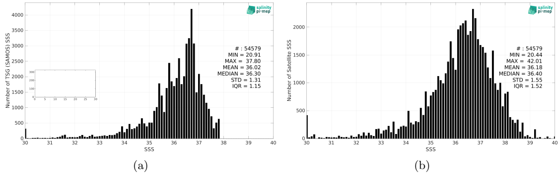
Figure 2: Histograms of SSS from TSG (SAMOS) (a) and SMOS SSS L2Q v331 - With FLAG (CMEMS-CATDS-CPDC) (b) considering all match-up pairs per bins of 0.1 over the Amazon and Orinoco river plumes Pi-MEP region and for the full satellite product period.
