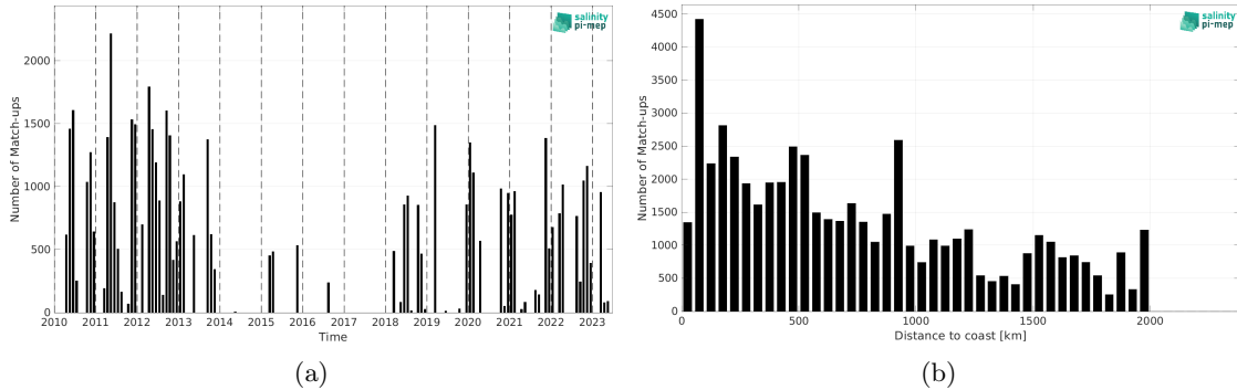
Figure 1: Number of match-ups between TSG (SAMOS) and SMOS SSS L2Q v331 - With FLAG (CMEMS-CATDS-CPDC) SSS as a function of time (a) and as function of the distance to coast (b) over the Amazon and Orinoco river plumes Pi-MEP region and for the full satellite product period.
