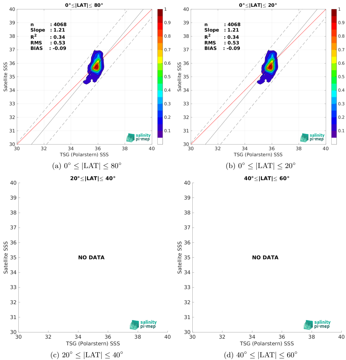
Figure 10: Contour maps of the concentration of SMOS SSS L2Q v331 - With FLAG (CMEMS-CATDS-CPDC) SSS (y-axis) versus TSG (Polarstern) SSS (x-axis) at match-up pairs for different latitude bands. For each plot, the red line shows x=y . The black thin and dashed lines indicate a linear fit through the data cloud and the \pm 95\% confidence levels, respectively. The number match-up pairs n , the slope and R^2 coefficient of the linear fit, the root mean square (RMS) and the mean bias between satellite and in situ data are indicated for each latitude band in each plots.
