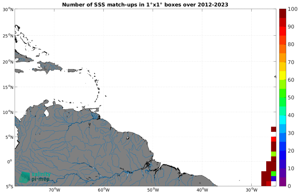
Figure 5: Number of SSS match-ups between TSG (Polarstern) SSS and the SMOS SSS L2Q v331 - With FLAG (CMEMS-CATDS-CPDC) SSS product for the Amazon and Orinoco river plumes Pi-MEP region over 1^\circ \times 1^\circ boxes and for the full satellite product period.
