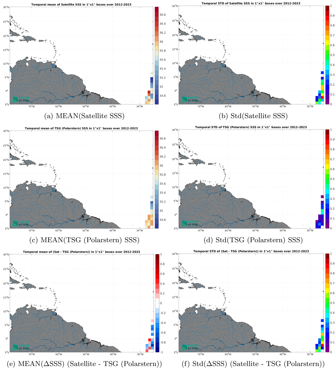
Figure 7: Temporal mean (left) and Std (right) of SSS from SMOS SSS L2Q v331 - With FLAG (CMEMS-CATDS-CPDC) (top), TSG (Polarstern) (middle), and of \Delta SSS (Satellite - TSG (Polarstern)). Only match-up pairs are used to generate these maps.
