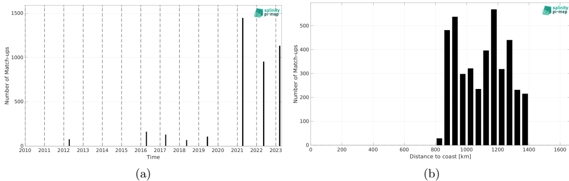
Figure 2: Number of match-ups between TSG (Polarstern) and SMOS SSS L2Q v331 - With FLAG (CMEMS-CATDS-CPDC) SSS as a function of time (a) and as function of the distance to coast (b) over the Amazon and Orinoco river plumes Pi-MEP region and for the full satellite product period.
