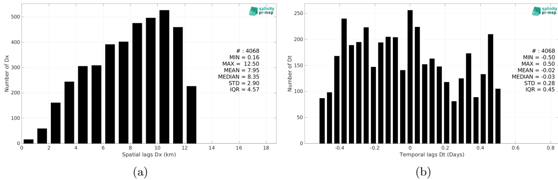
Figure 6: Histograms of the spatial (a) and temporal (b) lags between the location/time of the TSG (Polarstern) measurement and the date of the corresponding SMOS SSS L2Q v331 - With FLAG (CMEMS-CATDS-CPDC) SSS pixel.
