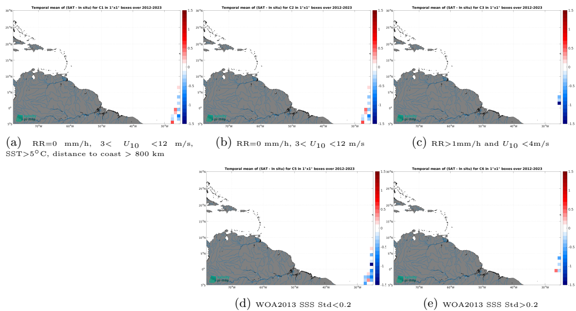
Figure 14: Temporal mean gridded over spatial boxes of size 1^\circ \times 1^\circ of \Delta SSS (SMOS SSS L2Q v331 - With FLAG (CMEMS-CATDS-CPDC) - TSG (Polarstern)) for 5 different subdatasets corresponding to:RR=0 mm/h, 3 < U_{10} < 12 m/s, SST >5^\circ C, distance to coast > 800 km (a), RR=0 mm/h, 3 < U_{10} < 12 m/s (b), RR >1 mm/h and U_{10} < 4 m/s (c), WOA2013 SSS Std <0.2 (d), WOA2013 SSS Std >0.2 (e).
