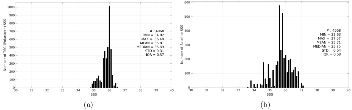
Figure 3: Histograms of SSS from TSG (Polarstern) (a) and SMOS SSS L2Q v331 - With FLAG (CMEMS-CATDS-CPDC) (b) considering all match-up pairs per bins of 0.1 over the Amazon and Orinoco river plumes Pi-MEP region and for the full satellite product period.
