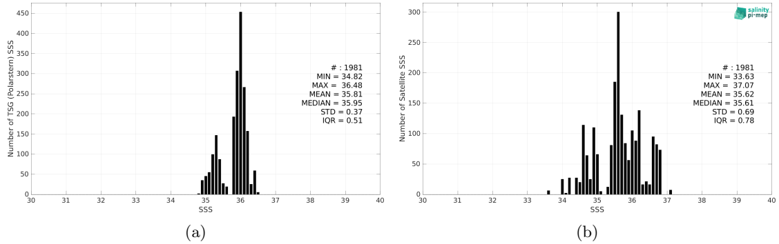
Figure 2: Histograms of SSS from TSG (Polarstern) (a) and SMOS SSS L2Q v331 - With FLAG (CMEMS-CATDS-CPDC) (b) considering all match-up pairs per bins of 0.1 over the Amazon and Orinoco river plumes Pi-MEP region and for the full satellite product period.
