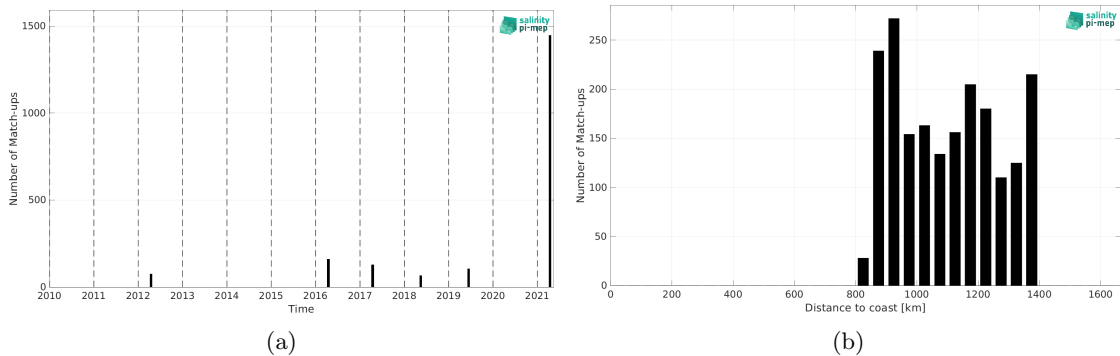
Figure 1: Number of match-ups between TSG (Polarstern) and SMOS SSS L2Q v331 - With FLAG (CMEMS-CATDS-CPDC) SSS as a function of time (a) and as function of the distance to coast (b) over the Amazon and Orinoco river plumes Pi-MEP region and for the full satellite product period.
