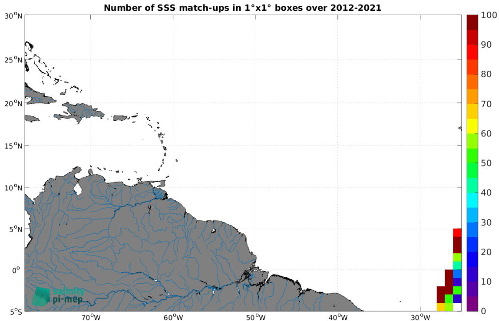
Figure 4: Number of SSS match-ups between TSG (Polarstern) SSS and the SMOS SSS L2Q v331 - With FLAG (CMEMS-CATDS-CPDC) SSS product for the Amazon and Orinoco river plumes Pi-MEP region over 1^\circ \times 1^\circ boxes and for the full satellite product period.
