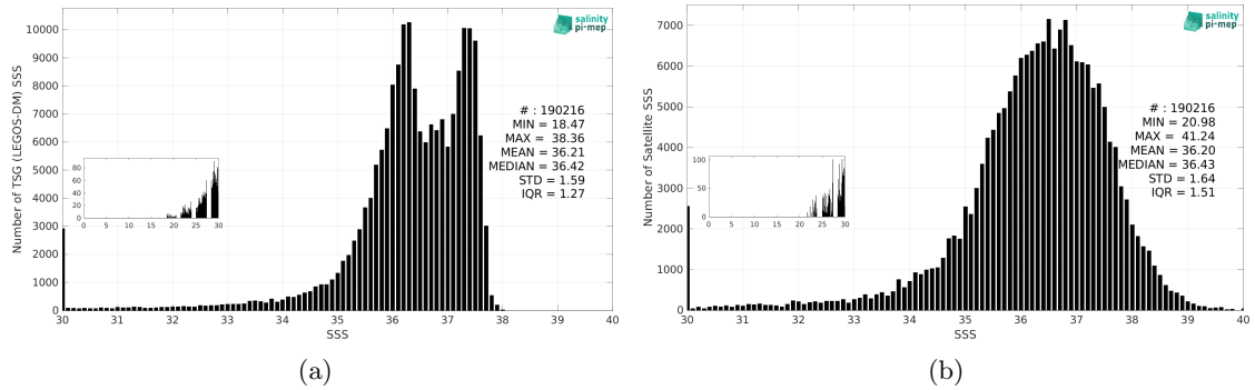
Figure 3: Histograms of SSS from TSG (LEGOS-DM) (a) and SMOS SSS L2Q v331 - With FLAG (CMEMS-CATDS-CPDC) (b) considering all match-up pairs per bins of 0.1 over the Amazon and Orinoco river plumes Pi-MEP region and for the full satellite product period.
