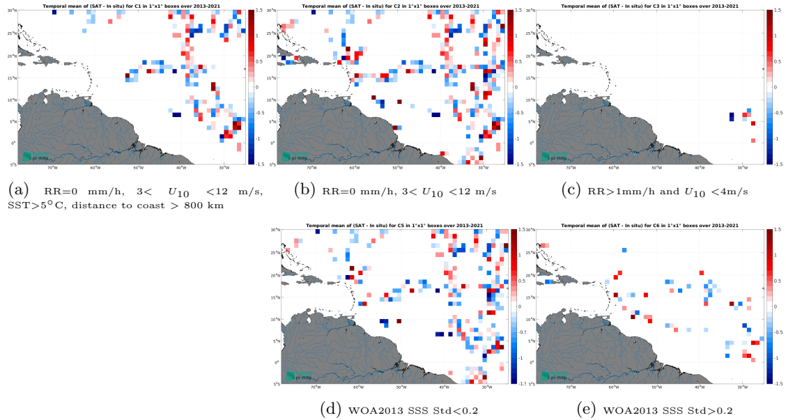
Figure 12: Temporal mean gridded over spatial boxes of size 1^{\circ}\times 1^{\circ} of \Delta SSS (SMOS SSS L2Q v331 - With FLAG (CMEMS-CATDS-CPDC) - TSG (GOSUD-Sailing-ship)) for 5 different subdatasets corresponding to:RR=0 mm/h, 3 < U_{10} < 12 m/s, SST >5^{\circ}\text{C} , distance to coast > 800 km (a), RR=0 mm/h, 3 < U_{10} < 12 m/s (b), RR >1 mm/h and U_{10} < 4 m/s (c), WOA2013 SSS Std <0.2 (d), WOA2013 SSS Std >0.2 (e).
