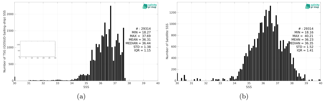
Figure 2: Histograms of SSS from TSG (GOSUD-Sailing-ship) (a) and SMOS SSS L2Q v331 - With FLAG (CMEMS-CATDS-CPDC) (b) considering all match-up pairs per bins of 0.1 over the Amazon and Orinoco river plumes Pi-MEP region and for the full satellite product period.
