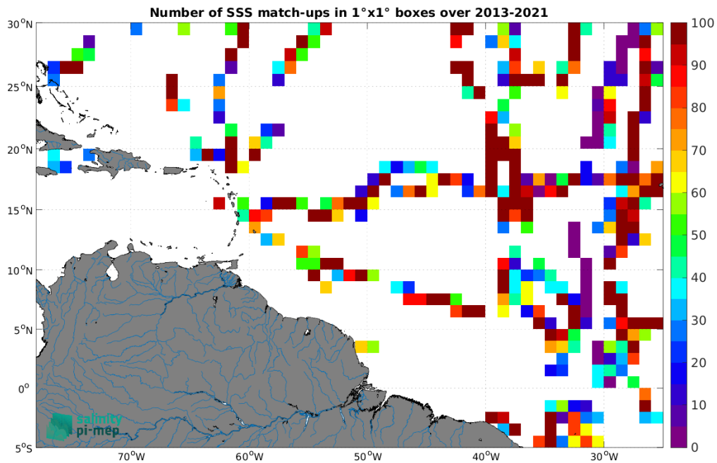
Figure 4: Number of SSS match-ups between TSG (GOSUD-Sailing-ship) SSS and the SMOS SSS L2Q v331 - With FLAG (CMEMS-CATDS-CPDC) SSS product for the Amazon and Orinoco river plumes Pi-MEP region over 1^\circ \times 1^\circ boxes and for the full satellite product period.
