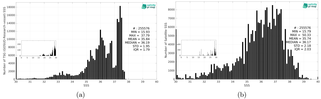
Figure 3: Histograms of SSS from TSG (GOSUD-Research-vessel) (a) and SMOS SSS L2Q v331 - With FLAG (CMEMS-CATDS-CPDC) (b) considering all match-up pairs per bins of 0.1 over the Amazon and Orinoco river plumes Pi-MEP region and for the full satellite product period.
