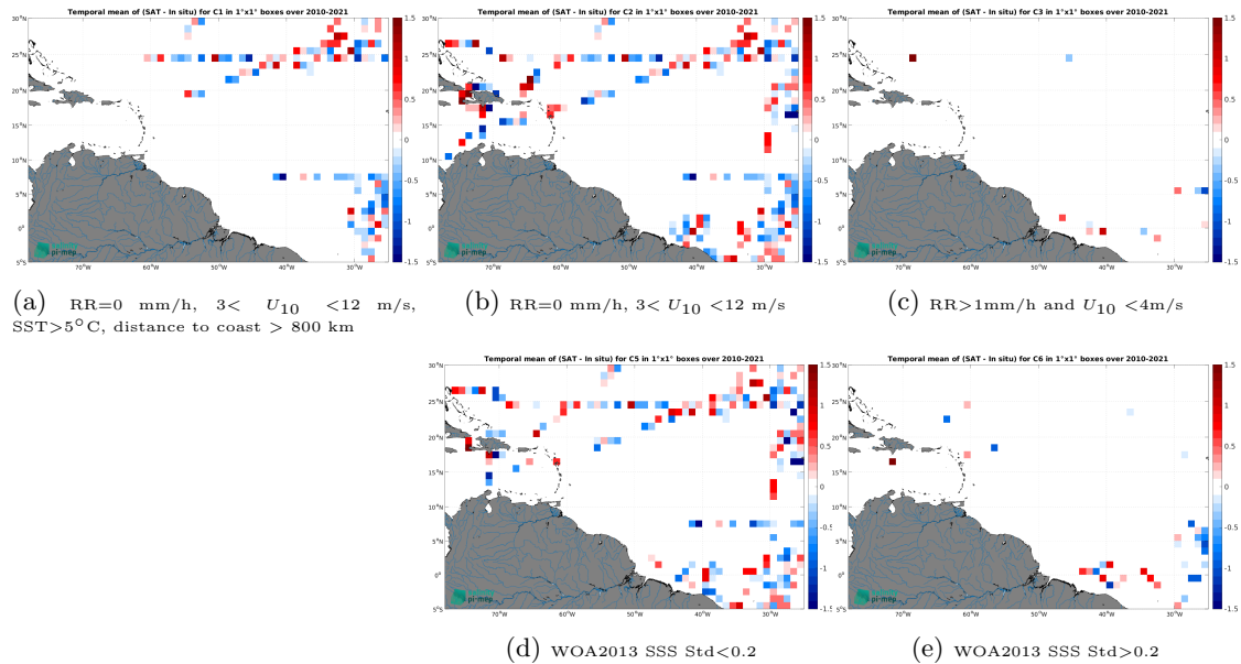
Figure 12: Temporal mean gridded over spatial boxes of size 1^{\circ}\times 1^{\circ} of \Delta\text{SSS} (SMOS SSS L2Q v331 - With FLAG (CMEMS-CATDS-CPDC) - TSG (CSIC-UTM)) for 5 different subdatasets corresponding to:RR=0 mm/h, 3 < U_{10} < 12 m/s, SST >5^{\circ}\text{C} , distance to coast > 800 km (a), RR=0 mm/h, 3 < U_{10} < 12 m/s (b), RR >1 mm/h and U_{10} < 4 m/s (c), WOA2013 SSS Std <0.2 (d), WOA2013 SSS Std >0.2 (e).
