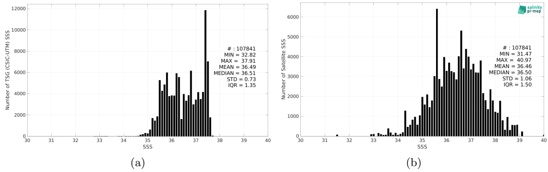
Figure 2: Histograms of SSS from TSG (CSIC-UTM) (a) and SMOS SSS L2Q v331 - With FLAG (CMEMS-CATDS-CPDC) (b) considering all match-up pairs per bins of 0.1 over the Amazon and Orinoco river plumes Pi-MEP region and for the full satellite product period.
