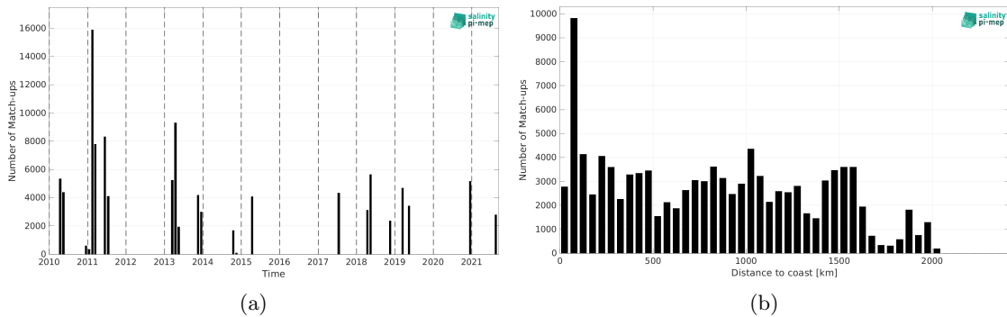
Figure 1: Number of match-ups between TSG (CSIC-UTM) and SMOS SSS L2Q v331 - With FLAG (CMEMS-CATDS-CPDC) SSS as a function of time (a) and as function of the distance to coast (b) over the Amazon and Orinoco river plumes Pi-MEP region and for the full satellite product period.
