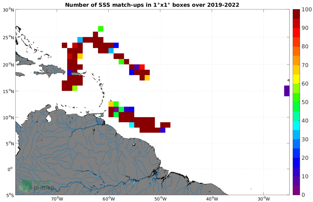
Figure 4: Number of SSS match-ups between Saildrone SSS and the SMOS SSS L2Q v331 - With FLAG (CMEMS-CATDS-CPDC) SSS product for the Amazon and Orinoco river plumes Pi-MEP region over 1^\circ \times 1^\circ boxes and for the full satellite product period.
