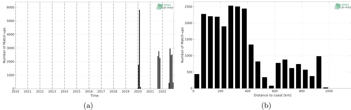
Figure 1: Number of match-ups between Saildrone and SMOS SSS L2Q v331 - With FLAG (CMEMS-CATDS-CPDC) SSS as a function of time (a) and as function of the distance to coast (b) over the Amazon and Orinoco river plumes Pi-MEP region and for the full satellite product period.
