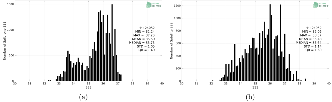
Figure 2: Histograms of SSS from Saildrone (a) and SMOS SSS L2Q v331 - With FLAG (CMEMS-CATDS-CPDC) (b) considering all match-up pairs per bins of 0.1 over the Amazon and Orinoco river plumes Pi-MEP region and for the full satellite product period.
