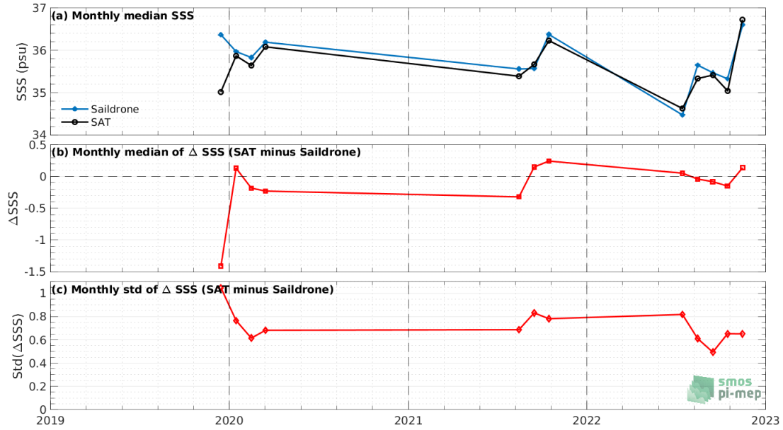
Figure 7: Time series of the monthly median SSS (top), median of \Delta SSS (Satellite - Sailldrone) and Std of \Delta SSS (Satellite - Sailldrone) over the Amazon and Orinoco river plumes Pi-MEP region considering all match-ups collected by the Pi-MEP.
