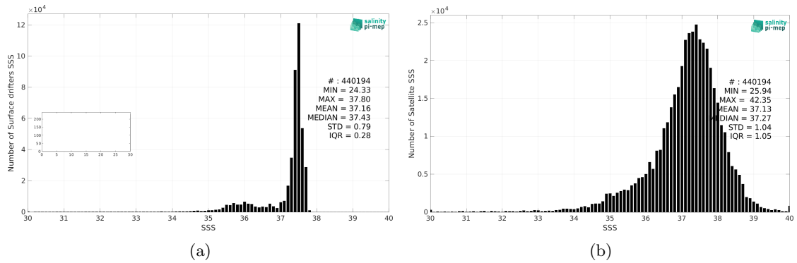
Figure 2: Histograms of SSS from Surface drifters (a) and SMOS SSS L2Q v331 - With FLAG (CMEMS-CATDS-CPDC) (b) considering all match-up pairs per bins of 0.1 over the Amazon and Orinoco river plumes Pi-MEP region and for the full satellite product period.
