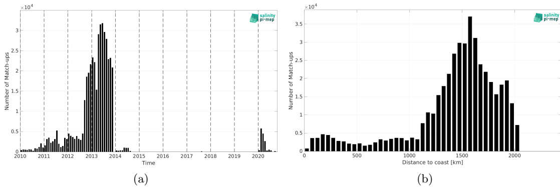
Figure 1: Number of match-ups between Surface drifters and SMOS SSS L2Q v331 - With FLAG (CMEMS-CATDS-CPDC) SSS as a function of time (a) and as function of the distance to coast (b) over the Amazon and Orinoco river plumes Pi-MEP region and for the full satellite product period.
