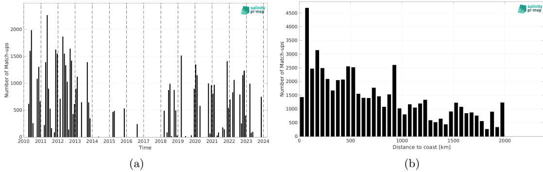
Figure 2: Number of match-ups between TSG (SAMOS) and SMOS SSS L2Q v331 - No FLAG (CMEMS-CATDS-CPDC) SSS as a function of time (a) and as function of the distance to coast (b) over the Amazon and Orinoco river plumes Pi-MEP region and for the full satellite product period.
