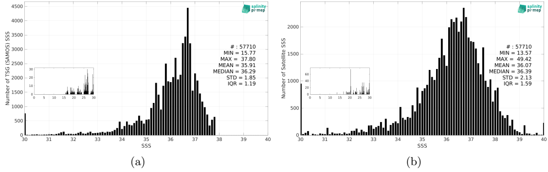
Figure 3: Histograms of SSS from TSG (SAMOS) (a) and SMOS SSS L2Q v331 - No FLAG (CMEMS-CATDS-CPDC) (b) considering all match-up pairs per bins of 0.1 over the Amazon and Orinoco river plumes Pi-MEP region and for the full satellite product period.
