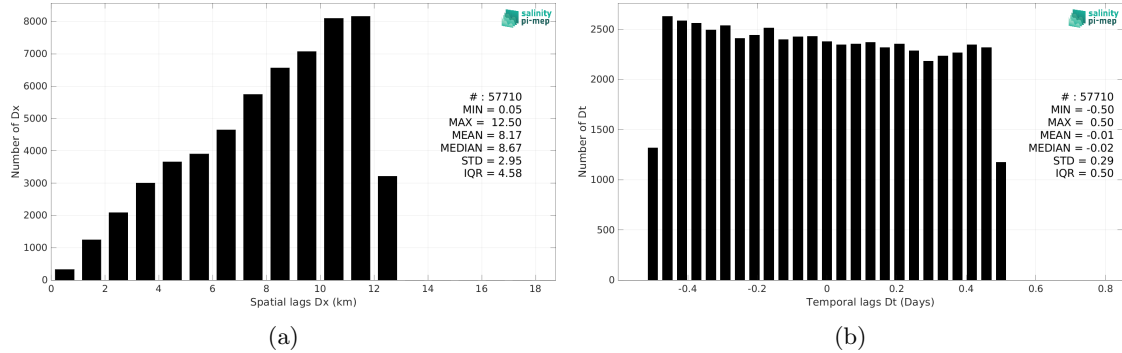
Figure 6: Histograms of the spatial (a) and temporal (b) lags between the location/time of the TSG (SAMOS) measurement and the date of the corresponding SMOS SSS L2Q v331 - No FLAG (CMEMS-CATDS-CPDC) SSS pixel.
