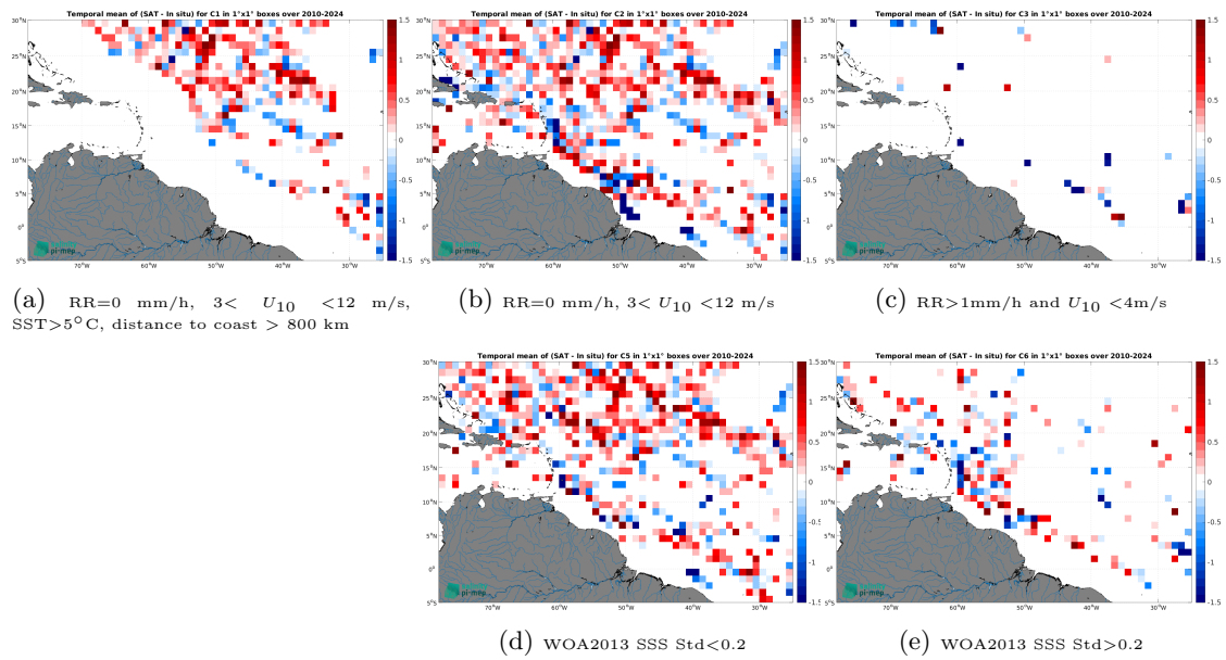
Figure 14: Temporal mean gridded over spatial boxes of size 1^\circ \times 1^\circ of \Delta SSS (SMOS SSS L2Q v331 - No FLAG (CMEMS-CATDS-CPDC) - TSG (SAMOS)) for 5 different subdatasets corresponding to: RR=0 mm/h, 3 < U_{10} < 12 m/s, SST > 5^\circ C , distance to coast > 800 km (a), RR=0 mm/h, 3 < U_{10} < 12 m/s (b), RR > 1 mm/h and U_{10} < 4 m/s (c), WOA2013 SSS Std < 0.2 (d), WOA2013 SSS Std > 0.2 (e).
