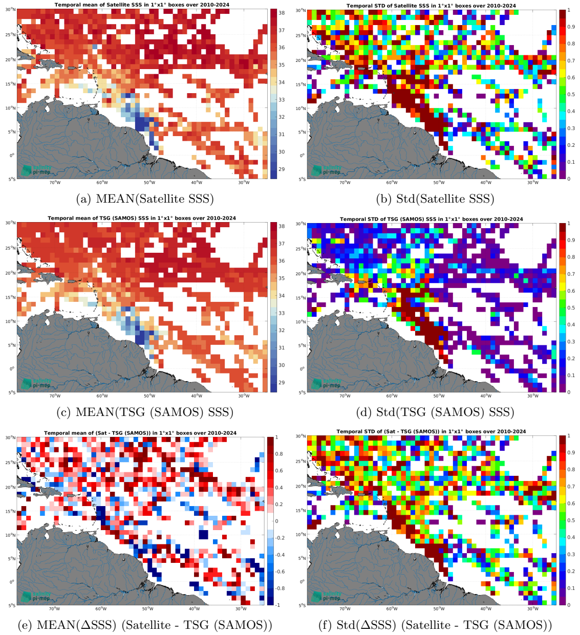
Figure 7: Temporal mean (left) and Std (right) of SSS from SMOS SSS L2Q v331 - No FLAG (CMEMS-CATDS-CPDC) (top), TSG (SAMOS) (middle), and of \Delta SSS (Satellite - TSG (SAMOS)). Only match-up pairs are used to generate these maps.
