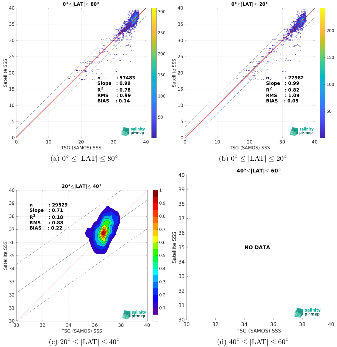
Figure 10: Contour maps of the concentration of SMOS SSS L2Q v331 - No FLAG (CMEMS-CATDS-CPDC) SSS (y-axis) versus TSG (SAMOS) SSS (x-axis) at match-up pairs for different latitude bands. For each plot, the red line shows x=y . The black thin and dashed lines indicate a linear fit through the data cloud and the \pm 95\% confidence levels, respectively. The number match-up pairs n , the slope and R^2 coefficient of the linear fit, the root mean square (RMS) and the mean bias between satellite and in situ data are indicated for each latitude band in each plots.
