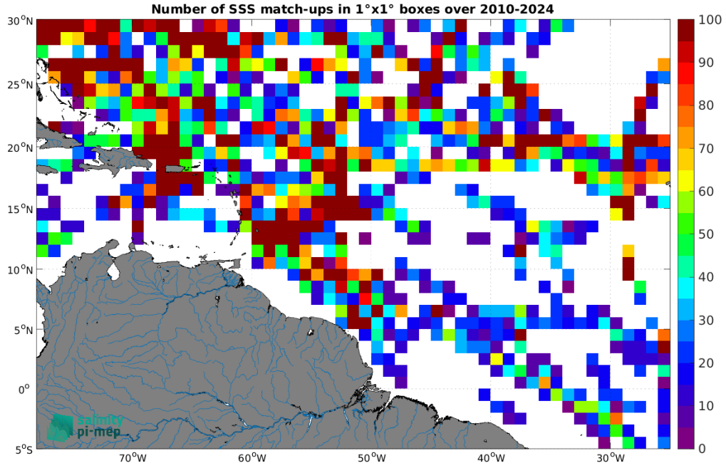
Figure 5: Number of SSS match-ups between TSG (SAMOS) SSS and the SMOS SSS L2Q v331 - No FLAG (CMEMS-CATDS-CPDC) SSS product for the Amazon and Orinoco river plumes Pi-MEP region over 1^\circ \times 1^\circ boxes and for the full satellite product period.
