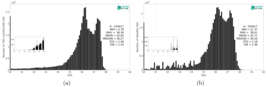
Figure 3: Histograms of SSS from TSG (LEGOS-DM) (a) and SMOS SSS L3 v9 - 9 Days (CATDS-CEC-LOCEAN) (b) considering all match-up pairs per bins of 0.1 over the Amazon and Orinoco river plumes Pi-MEP region and for the full satellite product period.
