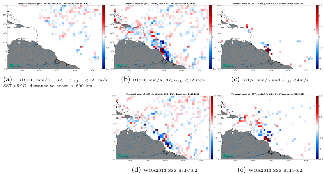
Figure 14: Temporal mean gridded over spatial boxes of size 1^\circ \times 1^\circ of \Delta SSS (SMOS SSS L3 v9 - 9 Days (CATDS-CEC-LOCEAN) - TSG (GOSUD-Research-vessel)) for 5 different subdatasets corresponding to:RR=0 mm/h, 3 < U_{10} < 12 m/s, SST >5^\circ C, distance to coast > 800 km (a), RR=0 mm/h, 3 < U_{10} < 12 m/s (b), RR >1 mm/h and U_{10} < 4 m/s (c), WOA2013 SSS Std <0.2 (d), WOA2013 SSS Std >0.2 (e).
