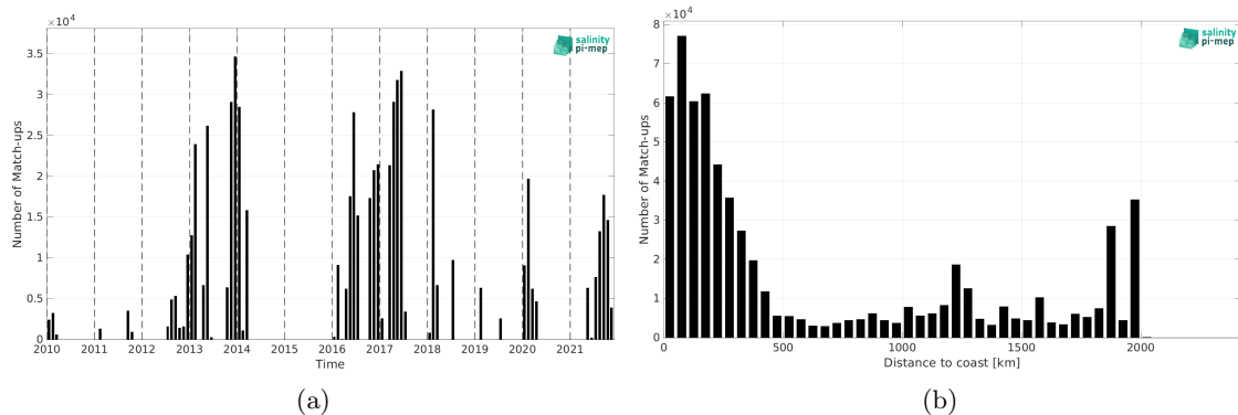
Figure 2: Number of match-ups between TSG (GOSUD-Research-vessel) and SMOS SSS L3 v9 - 9 Days (CATDS-CEC-LOCEAN) SSS as a function of time (a) and as function of the distance to coast (b) over the Amazon and Orinoco river plumes Pi-MEP region and for the full satellite product period.
