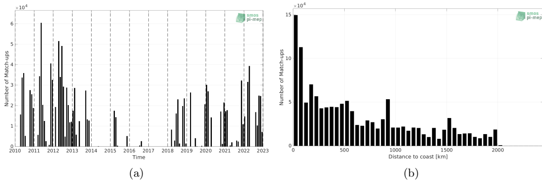
Figure 1: Number of match-ups between TSG (SAMOS) and SMOS SSS L3 v8 - 9 Days (CATDS-CECOS-LOCEAN) SSS as a function of time (a) and as function of the distance to coast (b) over the Amazon and Orinoco river plumes Pi-MEP region and for the full satellite product period.
