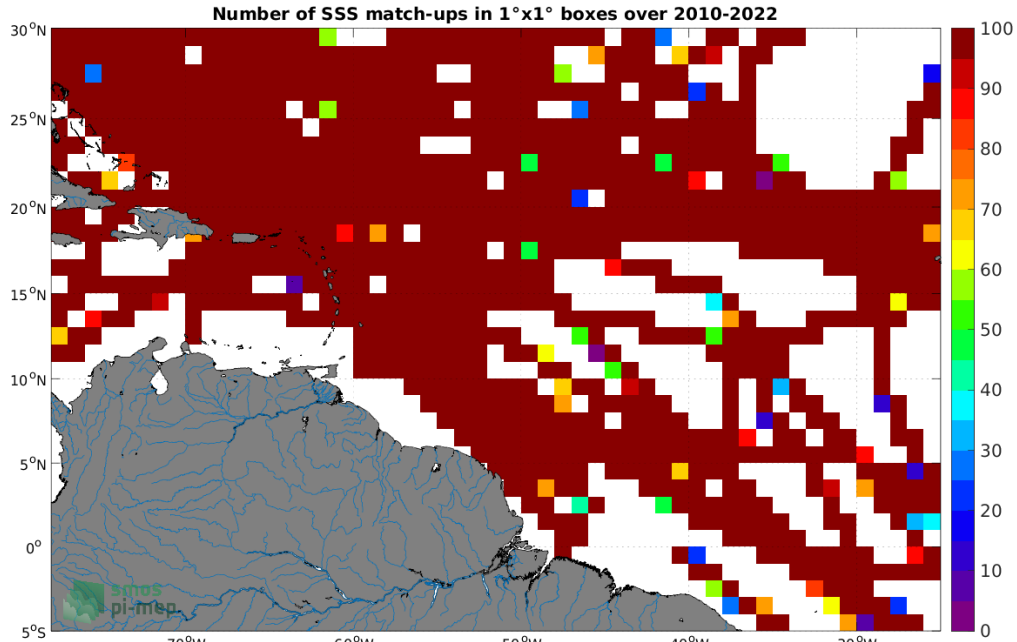
Figure 4: Number of SSS match-ups between TSG (SAMOS) SSS and the SMOS SSS L3 v8 - 9 Days (CATDS-CECOS-LOCEAN) SSS product for the Amazon and Orinoco river plumes Pi-MEP region over 1^\circ \times 1^\circ boxes and for the full satellite product period.
