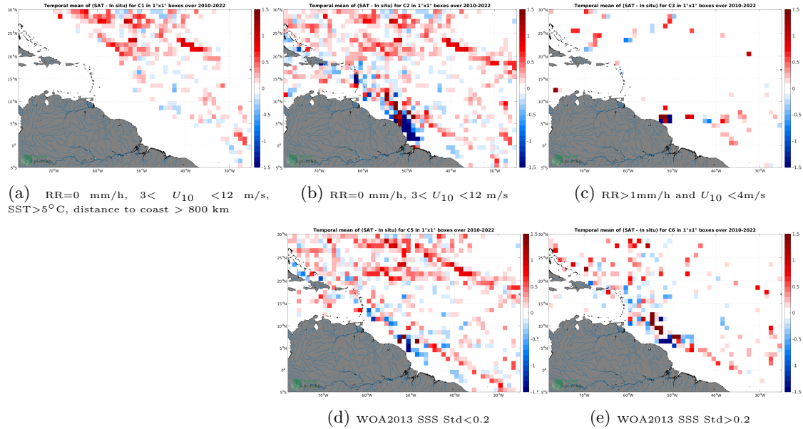
Figure 12: Temporal mean gridded over spatial boxes of size 1^{\circ}\times 1^{\circ} of \Delta\text{SSS} (SMOS SSS L3 v8 - 9 Days (CATDS-CECOS-LOCEAN) - TSG (SAMOS)) for 5 different subdatasets corresponding to:RR=0 mm/h, 3 < U_{10} < 12 m/s, SST >5^{\circ}\text{C} , distance to coast > 800 km (a), RR=0 mm/h, 3 < U_{10} < 12 m/s (b), RR >1 mm/h and U_{10} < 4 m/s (c), WOA2013 SSS Std <0.2 (d), WOA2013 SSS Std >0.2 (e).
