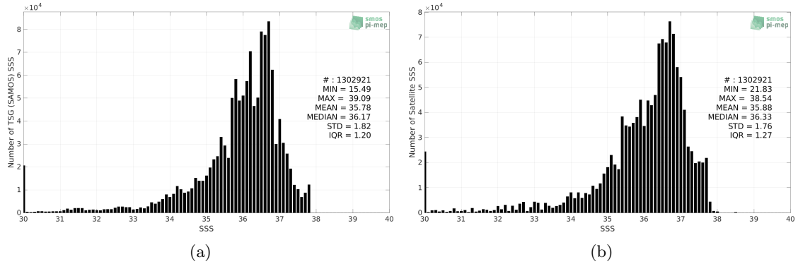
Figure 2: Histograms of SSS from TSG (SAMOS) (a) and SMOS SSS L3 v8 - 9 Days (CATDS-CECOS-LOCEAN) (b) considering all match-up pairs per bins of 0.1 over the Amazon and Orinoco river plumes Pi-MEP region and for the full satellite product period.
