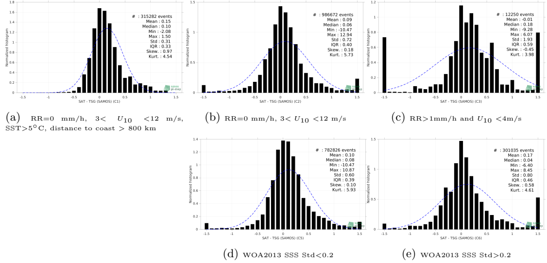
Figure 13: Normalized histogram of \Delta SSS (SMOS SSS L3 v8 - 9 Days (CATDS-CECOS-LOCEAN) - TSG (SAMOS)) for 5 different subdatasets corresponding to: RR=0 mm/h, 3 < U_{10} < 12 m/s, SST>5°C, distance to coast > 800 km (a), RR=0 mm/h, 3 < U_{10} < 12 m/s (b), RR>1mm/h and U_{10} < 4 m/s (c), WOA2013 SSS Std<0.2 (d), WOA2013 SSS Std>0.2 (e).
