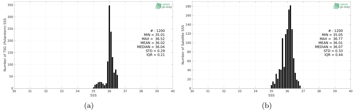
Figure 2: Histograms of SSS from TSG (Polarstern) (a) and SMOS SSS L3 v8 - 9 Days (CATDS-CECOS-LOCEAN) (b) considering all match-up pairs per bins of 0.1 over the Amazon and Orinoco river plumes Pi-MEP region and for the full satellite product period.
