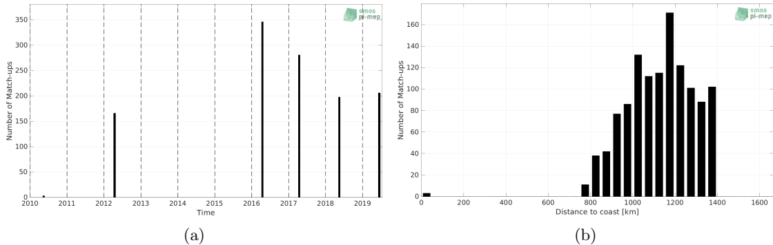
Figure 1: Number of match-ups between TSG (Polarstern) and SMOS SSS L3 v8 - 9 Days (CATDS-CECOS-LOCEAN) SSS as a function of time (a) and as function of the distance to coast (b) over the Amazon and Orinoco river plumes Pi-MEP region and for the full satellite product period.
