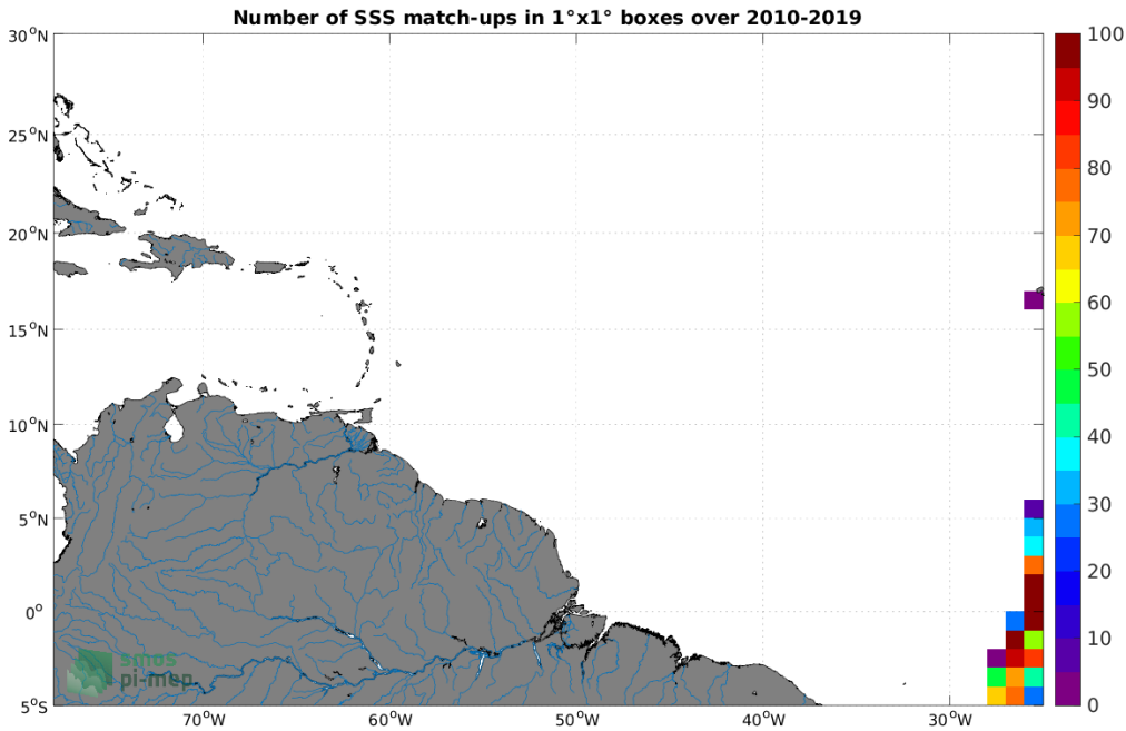
Figure 4: Number of SSS match-ups between TSG (Polarstern) SSS and the SMOS SSS L3 v8 - 9 Days (CATDS-CECOS-LOCEAN) SSS product for the Amazon and Orinoco river plumes Pi-MEP region over 1^\circ \times 1^\circ boxes and for the full satellite product period.
