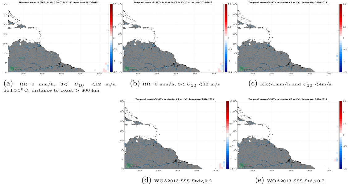
Figure 12: Temporal mean gridded over spatial boxes of size 1^{\circ}\times 1^{\circ} of \Delta\text{SSS} (SMOS SSS L3 v8 - 9 Days (CATDS-CECOS-LOCEAN) - TSG (Polarstern)) for 5 different subdatasets corresponding to:RR=0 mm/h, 3 < U_{10} < 12 m/s, SST >5^{\circ}\text{C} , distance to coast > 800 km (a), RR=0 mm/h, 3 < U_{10} < 12 m/s (b), RR >1 mm/h and U_{10} < 4 m/s (c), WOA2013 SSS Std <0.2 (d), WOA2013 SSS Std >0.2 (e).
