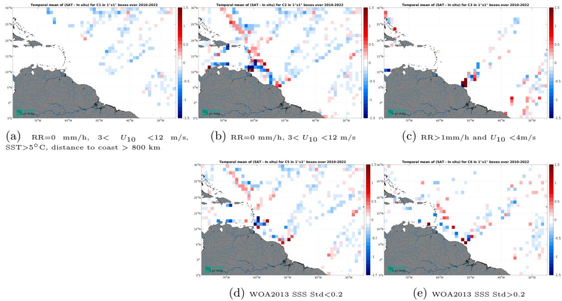
Figure 12: Temporal mean gridded over spatial boxes of size 1^\circ \times 1^\circ of \Delta SSS (SMOS SSS L3 v8 - 9 Days (CATDS-CEC-LOCEAN) - TSG (LEGOS-DM)) for 5 different subdatasets corresponding to:RR=0 mm/h, 3 < U_{10} < 12 m/s, SST >5^\circ C, distance to coast > 800 km (a), RR=0 mm/h, 3 < U_{10} < 12 m/s (b), RR >1 mm/h and U_{10} < 4 m/s (c), WOA2013 SSS Std <0.2 (d), WOA2013 SSS Std >0.2 (e).
