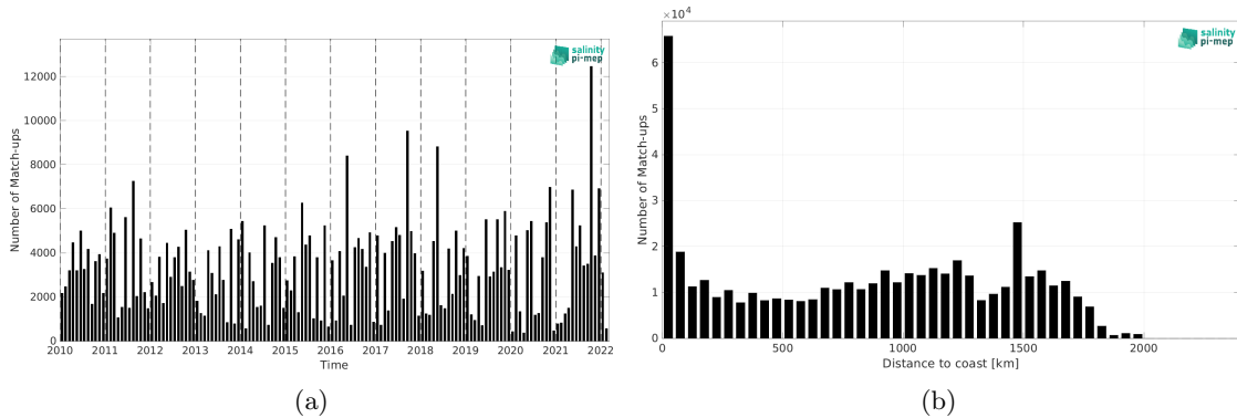
Figure 1: Number of match-ups between TSG (LEGOS-DM) and SMOS SSS L3 v8 - 9 Days (CATDS-CEC-LOCEAN) SSS as a function of time (a) and as function of the distance to coast (b) over the Amazon and Orinoco river plumes Pi-MEP region and for the full satellite product period.
