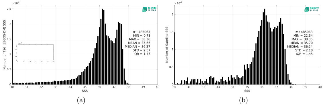
Figure 2: Histograms of SSS from TSG (LEGOS-DM) (a) and SMOS SSS L3 v8 - 9 Days (CATDS-CEC-LOCEAN) (b) considering all match-up pairs per bins of 0.1 over the Amazon and Orinoco river plumes Pi-MEP region and for the full satellite product period.
