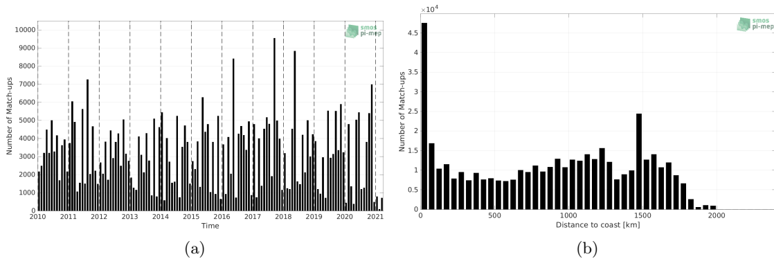
Figure 1: Number of match-ups between TSG (LEGOS-DM) and SMOS SSS L3 v8 - 9 Days (CATDS-CECOS-LOCEAN) SSS as a function of time (a) and as function of the distance to coast (b) over the Amazon and Orinoco river plumes Pi-MEP region and for the full satellite product period.
