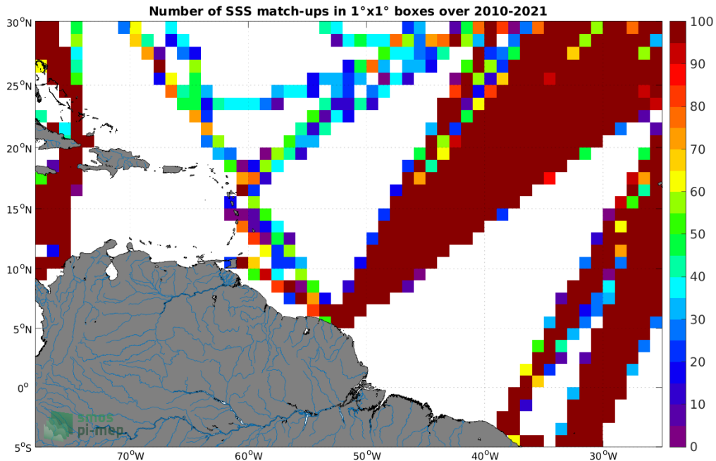
Figure 4: Number of SSS match-ups between TSG (LEGOS-DM) SSS and the SMOS SSS L3 v8 - 9 Days (CATDS-CECOS-LOCEAN) SSS product for the Amazon and Orinoco river plumes Pi-MEP region over 1^\circ \times 1^\circ boxes and for the full satellite product period.
