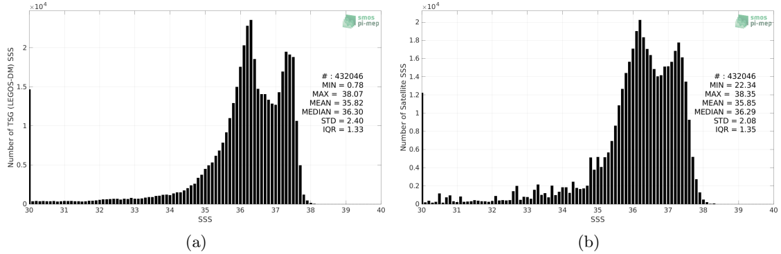
Figure 2: Histograms of SSS from TSG (LEGOS-DM) (a) and SMOS SSS L3 v8 - 9 Days (CATDS-CECOS-LOCEAN) (b) considering all match-up pairs per bins of 0.1 over the Amazon and Orinoco river plumes Pi-MEP region and for the full satellite product period.
