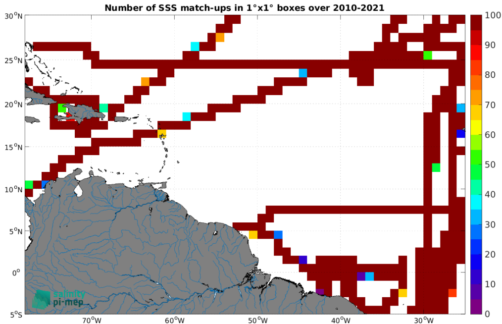
Figure 4: Number of SSS match-ups between TSG (CSIC-UTM) SSS and the SMOS SSS L3 v8 - 9 Days (CATDS-CEC-LOCEAN) SSS product for the Amazon and Orinoco river plumes Pi-MEP region over 1^\circ \times 1^\circ boxes and for the full satellite product period.
