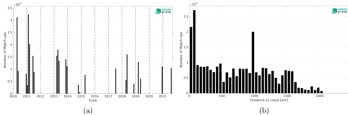
Figure 1: Number of match-ups between TSG (CSIC-UTM) and SMOS SSS L3 v8 - 9 Days (CATDS-CEC-LOCEAN) SSS as a function of time (a) and as function of the distance to coast (b) over the Amazon and Orinoco river plumes Pi-MEP region and for the full satellite product period.
