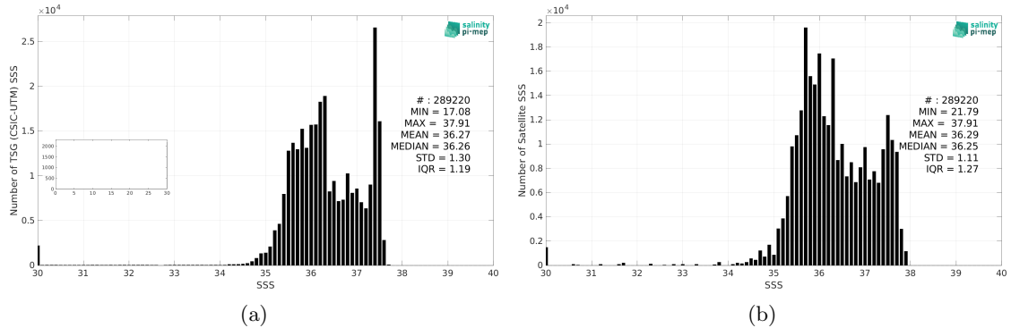
Figure 2: Histograms of SSS from TSG (CSIC-UTM) (a) and SMOS SSS L3 v8 - 9 Days (CATDS-CEC-LOCEAN) (b) considering all match-up pairs per bins of 0.1 over the Amazon and Orinoco river plumes Pi-MEP region and for the full satellite product period.
