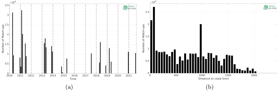
Figure 1: Number of match-ups between TSG (CSIC-UTM) and SMOS SSS L3 v8 - 9 Days (CATDS-CECOS-LOCEAN) SSS as a function of time (a) and as function of the distance to coast (b) over the Amazon and Orinoco river plumes Pi-MEP region and for the full satellite product period.
