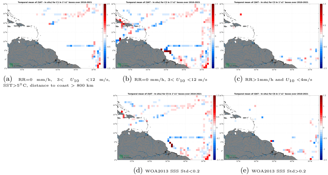
Figure 12: Temporal mean gridded over spatial boxes of size 1^{\circ}\times 1^{\circ} of \Delta\text{SSS} (SMOS SSS L3 v8 - 9 Days (CATDS-CECOS-LOCEAN) - TSG (CSIC-UTM)) for 5 different subdatasets corresponding to:RR=0 mm/h, 3 < U_{10} < 12 m/s, SST >5^{\circ}\text{C} , distance to coast > 800 km (a), RR=0 mm/h, 3 < U_{10} < 12 m/s (b), RR >1 mm/h and U_{10} < 4 m/s (c), WOA2013 SSS Std <0.2 (d), WOA2013 SSS Std >0.2 (e).
