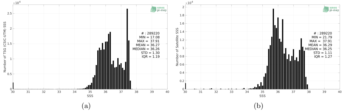
Figure 2: Histograms of SSS from TSG (CSIC-UTM) (a) and SMOS SSS L3 v8 - 9 Days (CATDS-CECOS-LOCEAN) (b) considering all match-up pairs per bins of 0.1 over the Amazon and Orinoco river plumes Pi-MEP region and for the full satellite product period.
