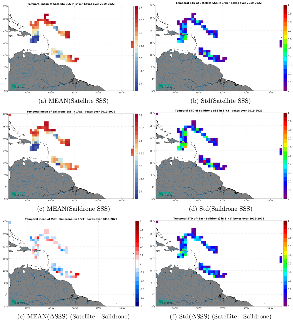
Figure 6: Temporal mean (left) and Std (right) of SSS from SMOS SSS L3 v8 - 9 Days (CATDS-CEC-LOCEAN) (top), Saildrone (middle), and of \Delta SSS (Satellite - Saildrone). Only match-up pairs are used to generate these maps.
