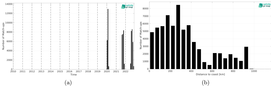
Figure 1: Number of match-ups between Saildrone and SMOS SSS L3 v8 - 9 Days (CATDS-CEC-LOCEAN) SSS as a function of time (a) and as function of the distance to coast (b) over the Amazon and Orinoco river plumes Pi-MEP region and for the full satellite product period.
