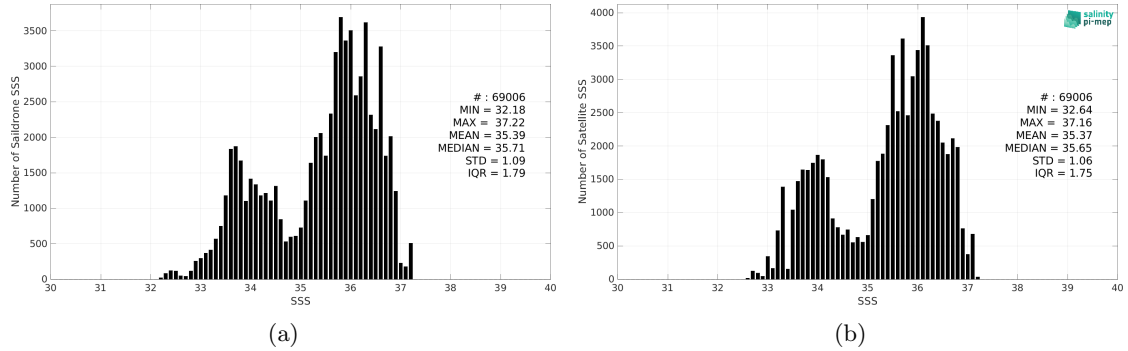
Figure 2: Histograms of SSS from Saildrone (a) and SMOS SSS L3 v8 - 9 Days (CATDS-CEC-LOCEAN) (b) considering all match-up pairs per bins of 0.1 over the Amazon and Orinoco river plumes Pi-MEP region and for the full satellite product period.
