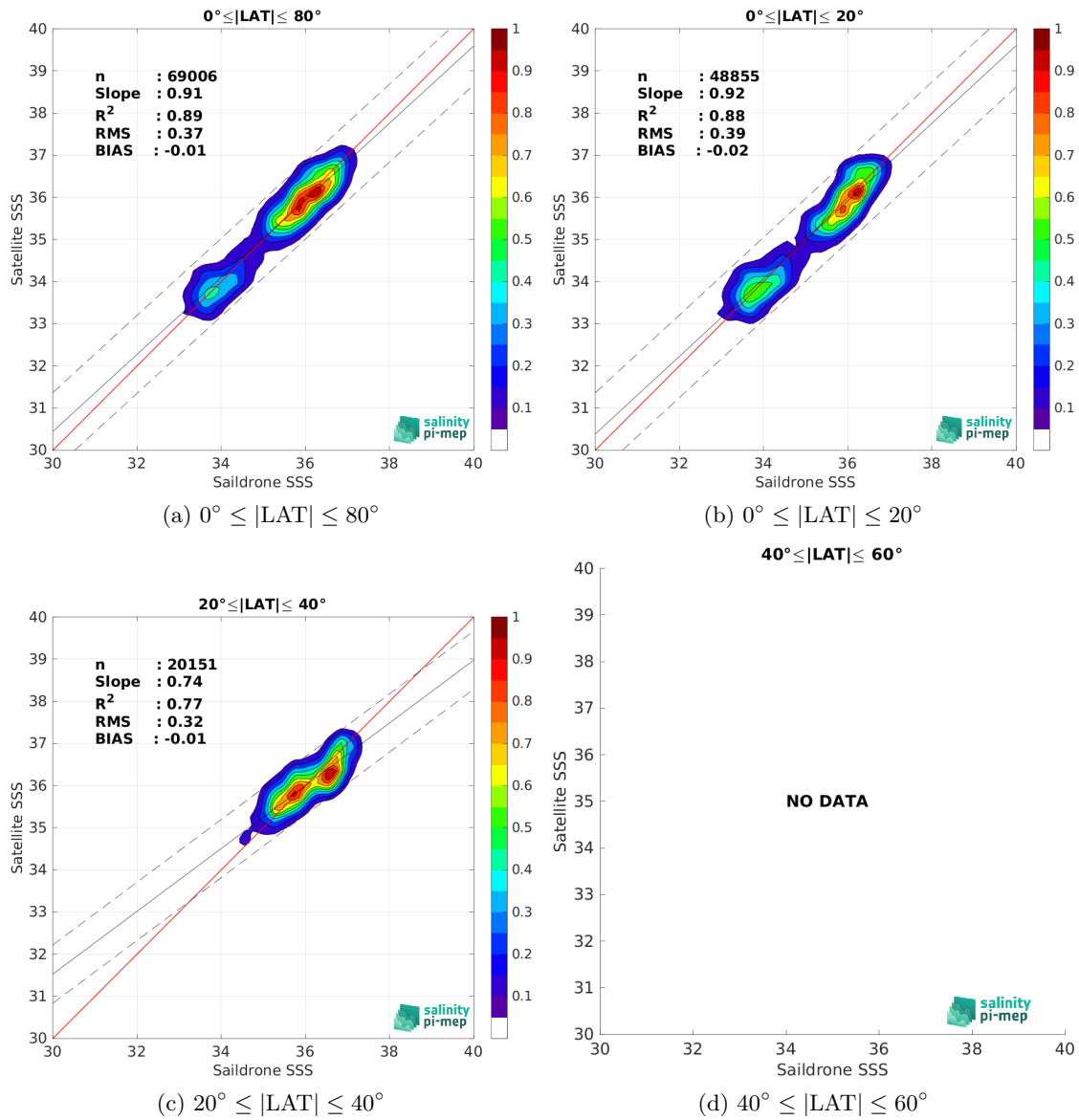
Figure 9: Contour maps of the concentration of SMOS SSS L3 v8 - 9 Days (CATDS-CEC-LOCEAN) SSS (y-axis) versus Sailldrone SSS (x-axis) at match-up pairs for different latitude bands. For each plot, the red line shows x=y . The black thin and dashed lines indicate a linear fit through the data cloud and the \pm 95\% confidence levels, respectively. The number match-up pairs n , the slope and R^2 coefficient of the linear fit, the root mean square (RMS) and the mean bias between satellite and in situ data are indicated for each latitude band in each plots.
