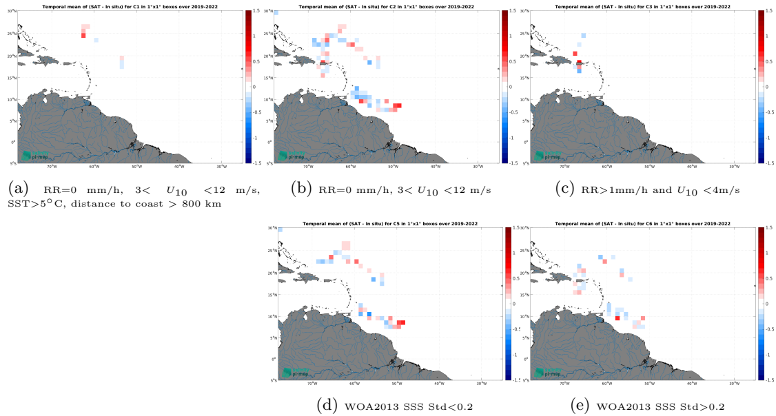
Figure 12: Temporal mean gridded over spatial boxes of size 1^\circ \times 1^\circ of \Delta SSS (SMOS SSS L3 v8 - 9 Days (CATDS-CEC-LOCEAN) - Saildrone) for 5 different subdatasets corresponding to:RR=0 mm/h, 3 < U_{10} < 12 m/s, SST >5^\circ\text{C} , distance to coast > 800 km (a), RR=0 mm/h, 3 < U_{10} < 12 m/s (b), RR >1 mm/h and U_{10} < 4 m/s (c), WOA2013 SSS Std <0.2 (d), WOA2013 SSS Std >0.2 (e).
