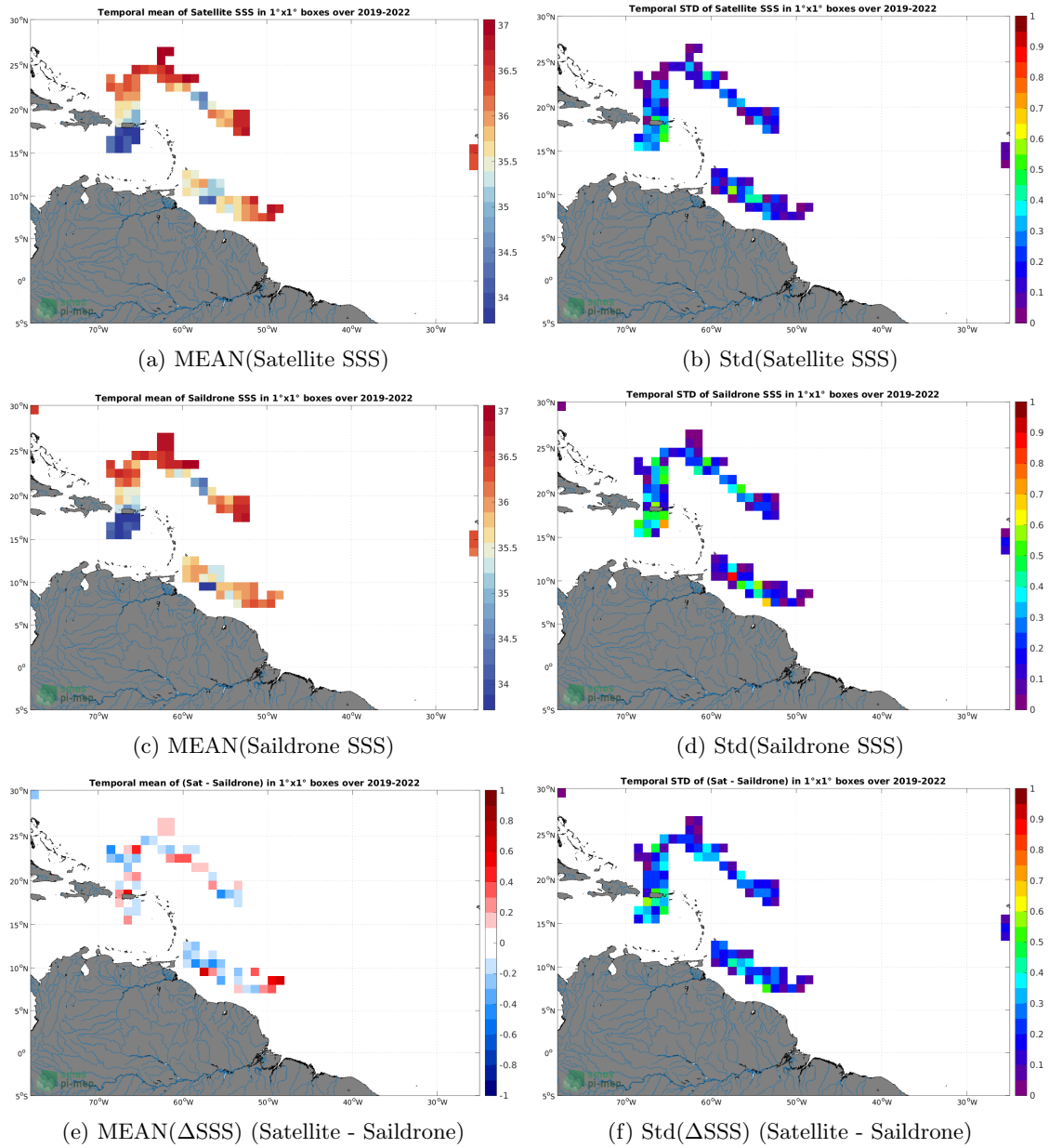
Figure 6: Temporal mean (left) and Std (right) of SSS from SMOS SSS L3 v8 - 9 Days (CATDS-CECOS-LOCEAN) (top), Saildrone (middle), and of \Delta SSS (Satellite - Saildrone). Only match-pairs are used to generate these maps.
