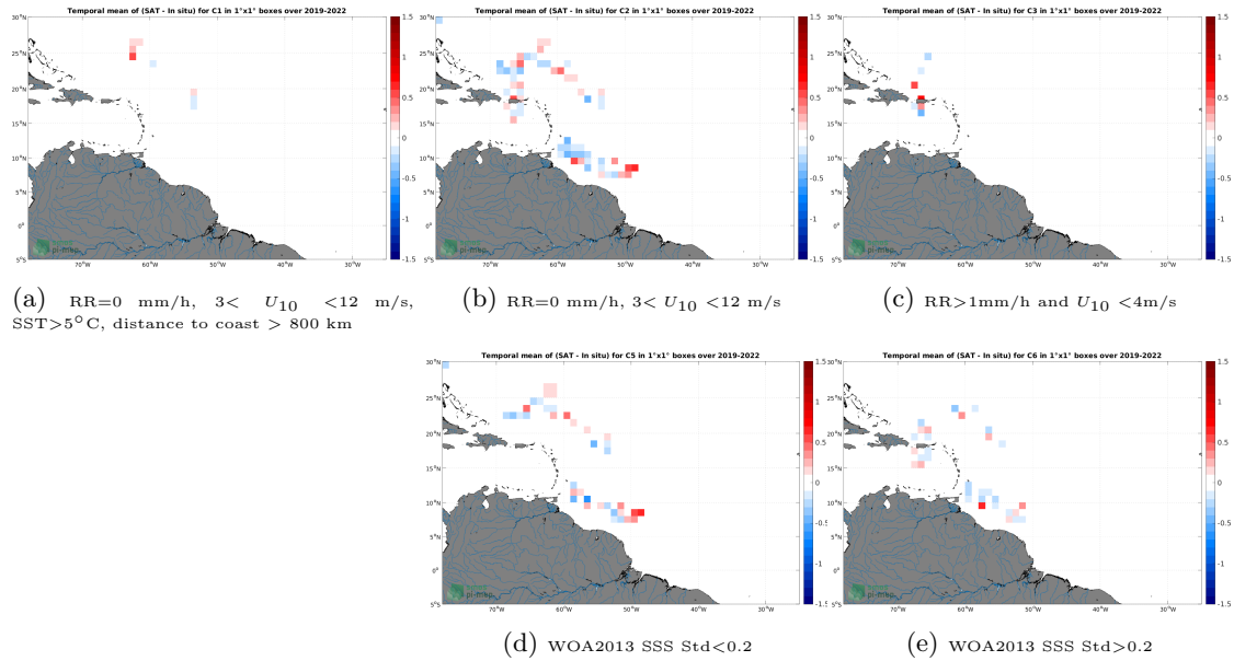
Figure 12: Temporal mean gridded over spatial boxes of size 1^\circ \times 1^\circ of \Delta SSS (SMOS SSS L3 v8 - 9 Days (CATDS-CECOS-LOCEAN) - Saildrone) for 5 different subdatasets corresponding to:RR=0 mm/h, 3 < U_{10} < 12 m/s, SST >5^\circ\text{C} , distance to coast > 800 km (a), RR=0 mm/h, 3 < U_{10} < 12 m/s (b), RR >1 mm/h and U_{10} < 4 m/s (c), WOA2013 SSS Std <0.2 (d), WOA2013 SSS Std >0.2 (e).
