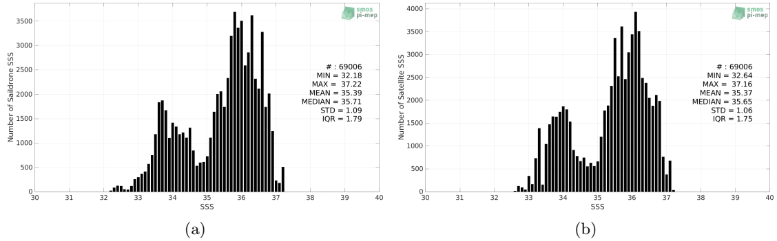
Figure 2: Histograms of SSS from Saildrone (a) and SMOS SSS L3 v8 - 9 Days (CATDS-CECOS-LOCEAN) (b) considering all match-up pairs per bins of 0.1 over the Amazon and Orinoco river plumes Pi-MEP region and for the full satellite product period.
