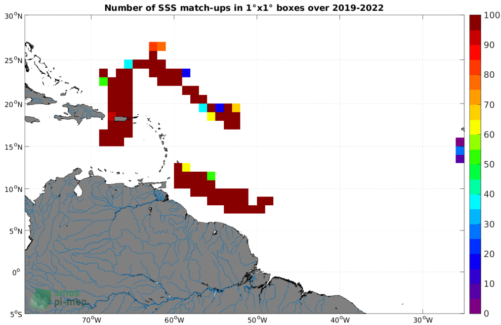
Figure 4: Number of SSS match-ups between Saildrone SSS and the SMOS SSS L3 v8 - 9 Days (CATDS-CECOS-LOCEAN) SSS product for the Amazon and Orinoco river plumes Pi-MEP region over 1^\circ \times 1^\circ boxes and for the full satellite product period.
