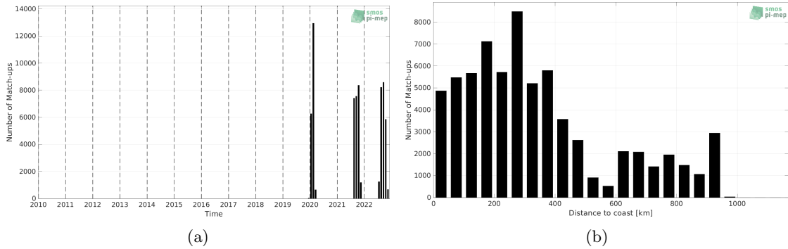
Figure 1: Number of match-ups between Sairdrone and SMOS SSS L3 v8 - 9 Days (CATDS-CECOS-LOCEAN) SSS as a function of time (a) and as function of the distance to coast (b) over the Amazon and Orinoco river plumes Pi-MEP region and for the full satellite product period.
