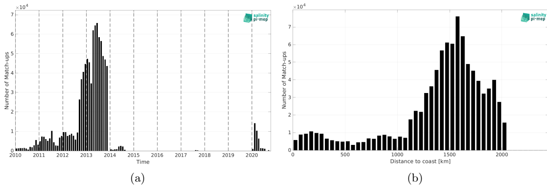
Figure 1: Number of match-ups between Surface drifters and SMOS SSS L3 v8 - 9 Days (CATDS-CEC-LOCEAN) SSS as a function of time (a) and as function of the distance to coast (b) over the Amazon and Orinoco river plumes Pi-MEP region and for the full satellite product period.
