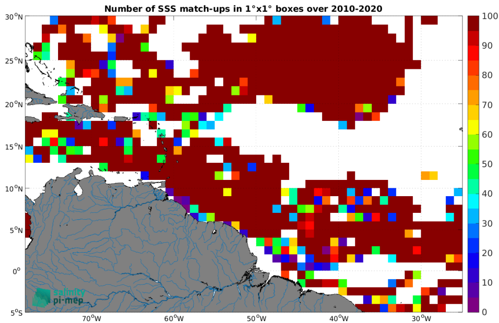
Figure 3: Number of SSS match-ups between Surface drifters SSS and the SMOS SSS L3 v8 - 9 Days (CATDS-CEC-LOCEAN) SSS product for the Amazon and Orinoco river plumes Pi-MEP region over 1^\circ \times 1^\circ boxes and for the full satellite product period.
