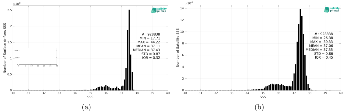
Figure 2: Histograms of SSS from Surface drifters (a) and SMOS SSS L3 v8 - 9 Days (CATDS-CEC-LOCEAN) (b) considering all match-up pairs per bins of 0.1 over the Amazon and Orinoco river plumes Pi-MEP region and for the full satellite product period.
